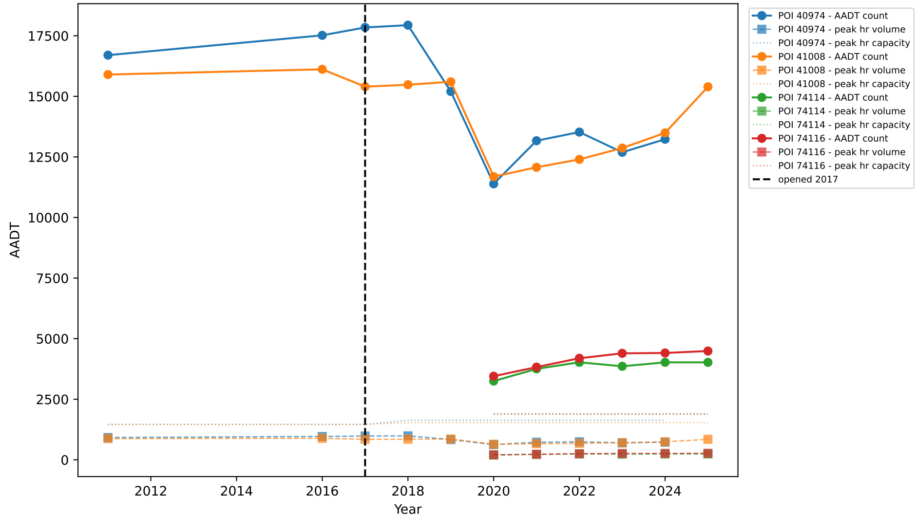
F-M-0436: Traffic Counts, Peak Volume & Capacity by Station
