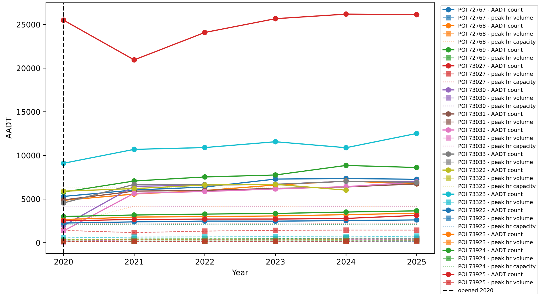
F-M-0507: Traffic Counts, Peak Volume & Capacity by Station
