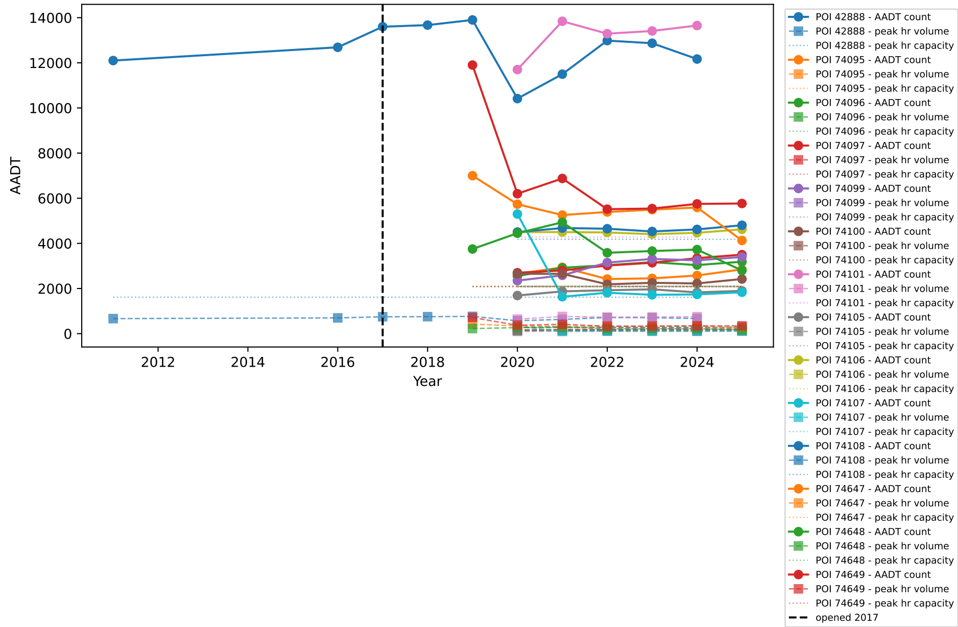
FM-0907: Traffic Counts, Peak Volume & Capacity by Station
