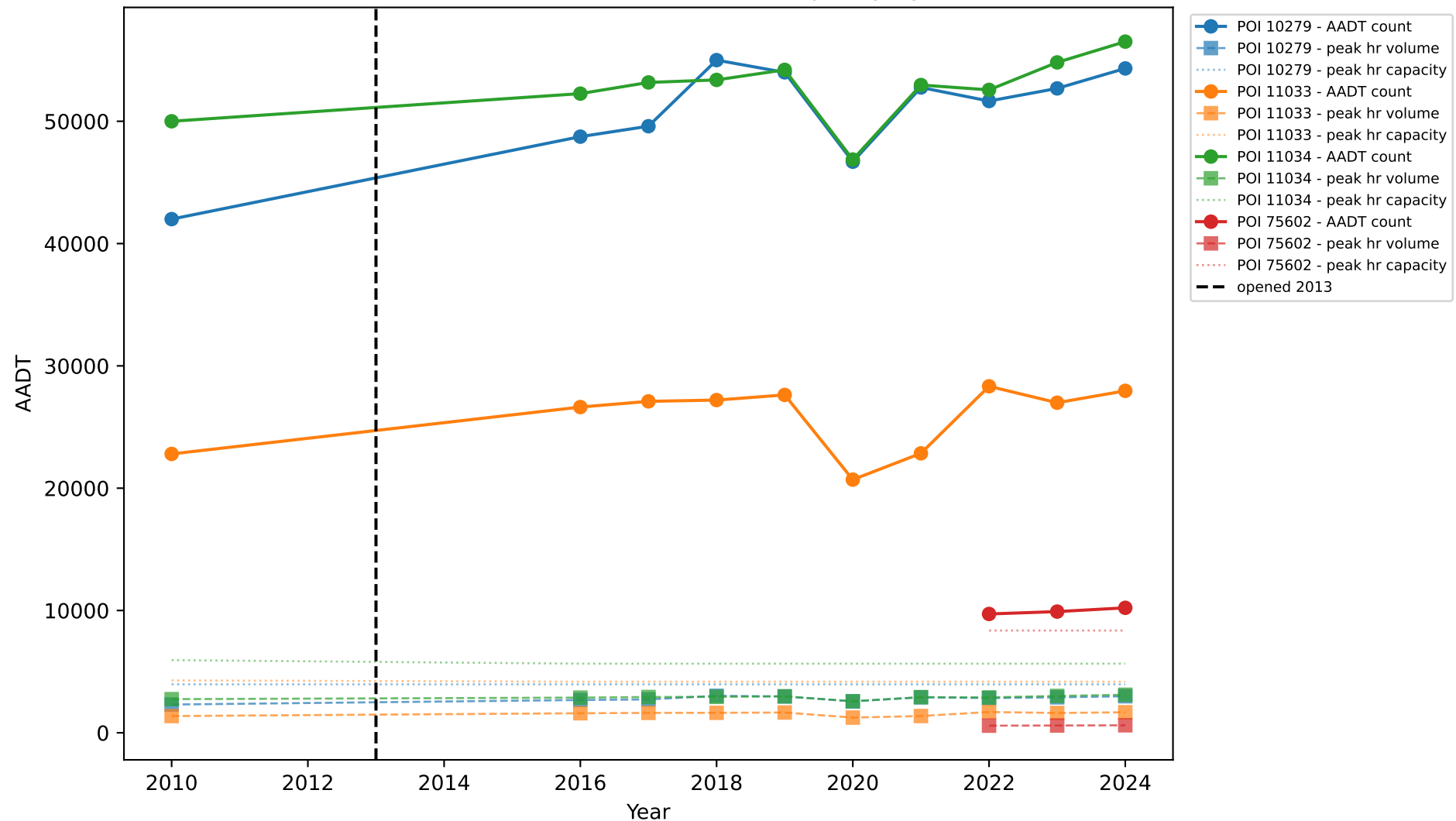
FM-0915: Traffic Counts, Peak Volume & Capacity by Station
