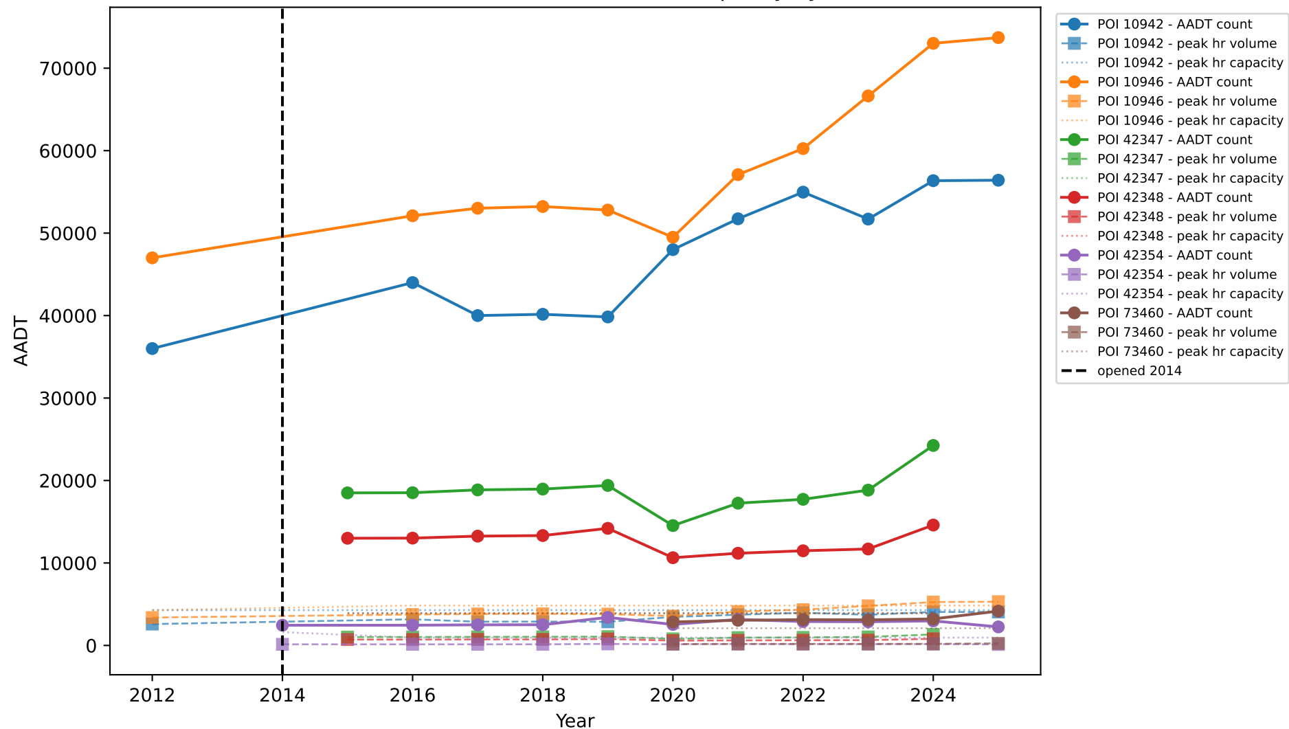
FM-1101: Traffic Counts, Peak Volume & Capacity by Station
