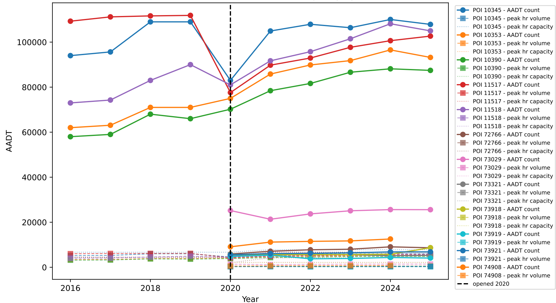
FM-1315: Traffic Counts, Peak Volume & Capacity by Station
