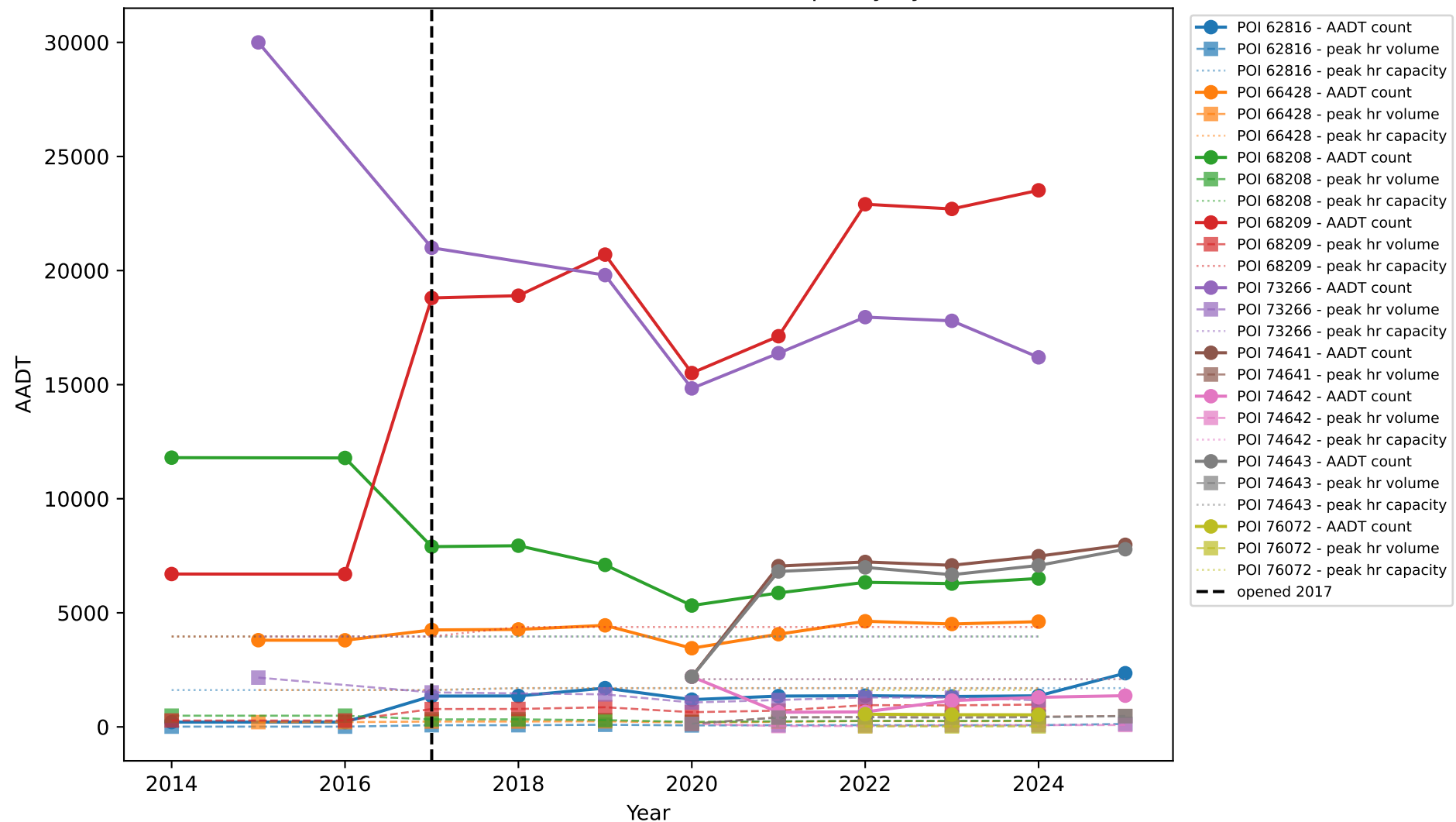
FM-1317: Traffic Counts, Peak Volume & Capacity by Station
