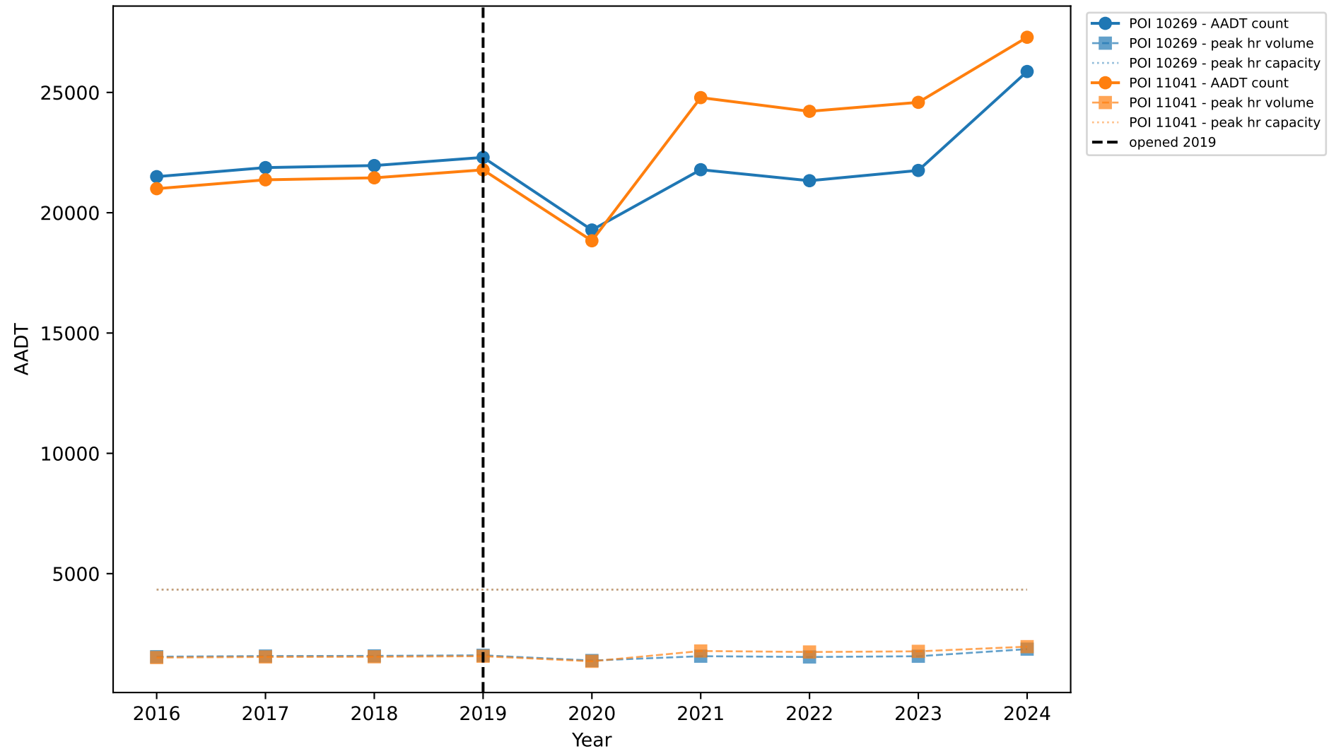
FM-1320: Traffic Counts, Peak Volume & Capacity by Station
