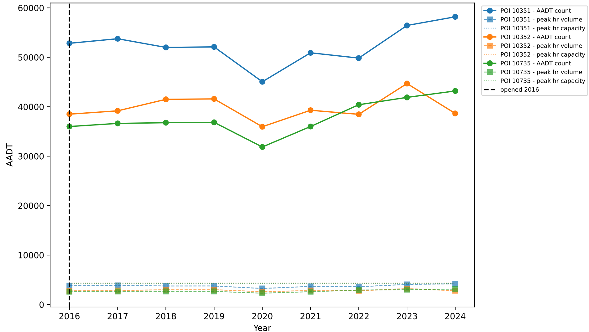
FM-1403: Traffic Counts, Peak Volume & Capacity by Station
