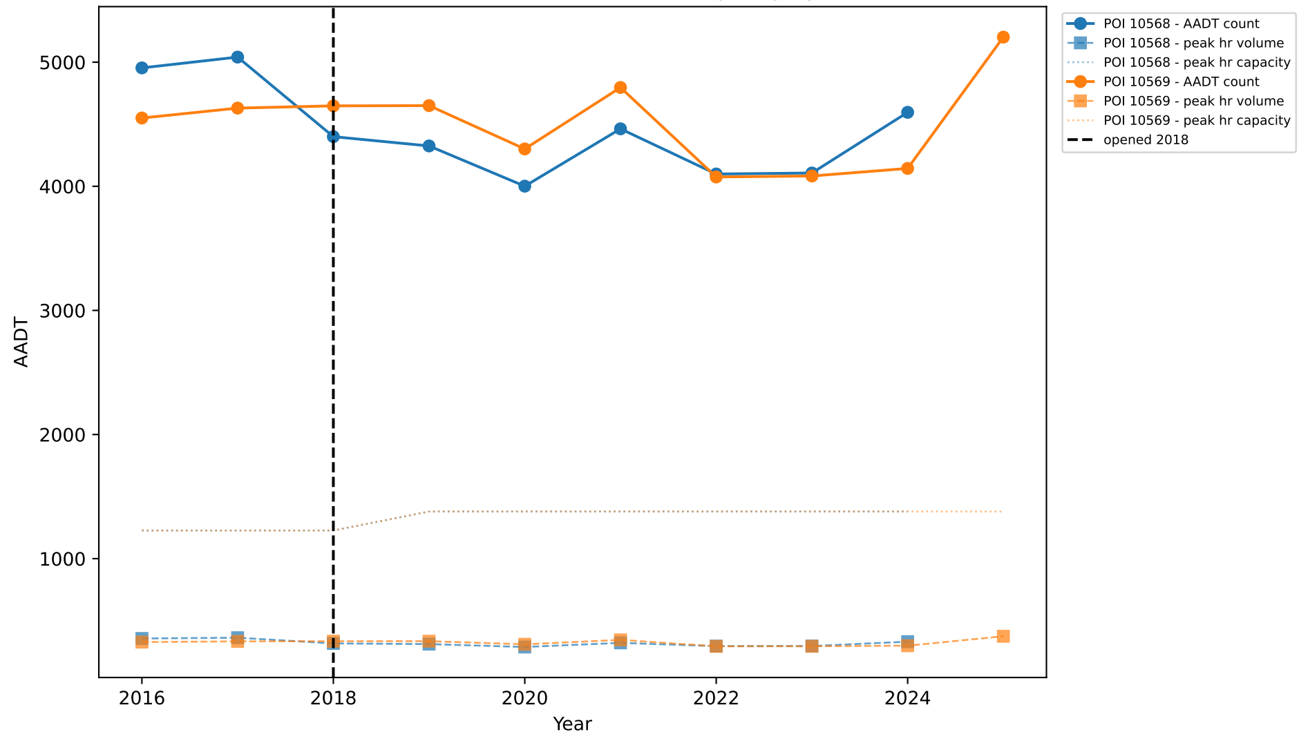
FM-1506: Traffic Counts, Peak Volume & Capacity by Station
