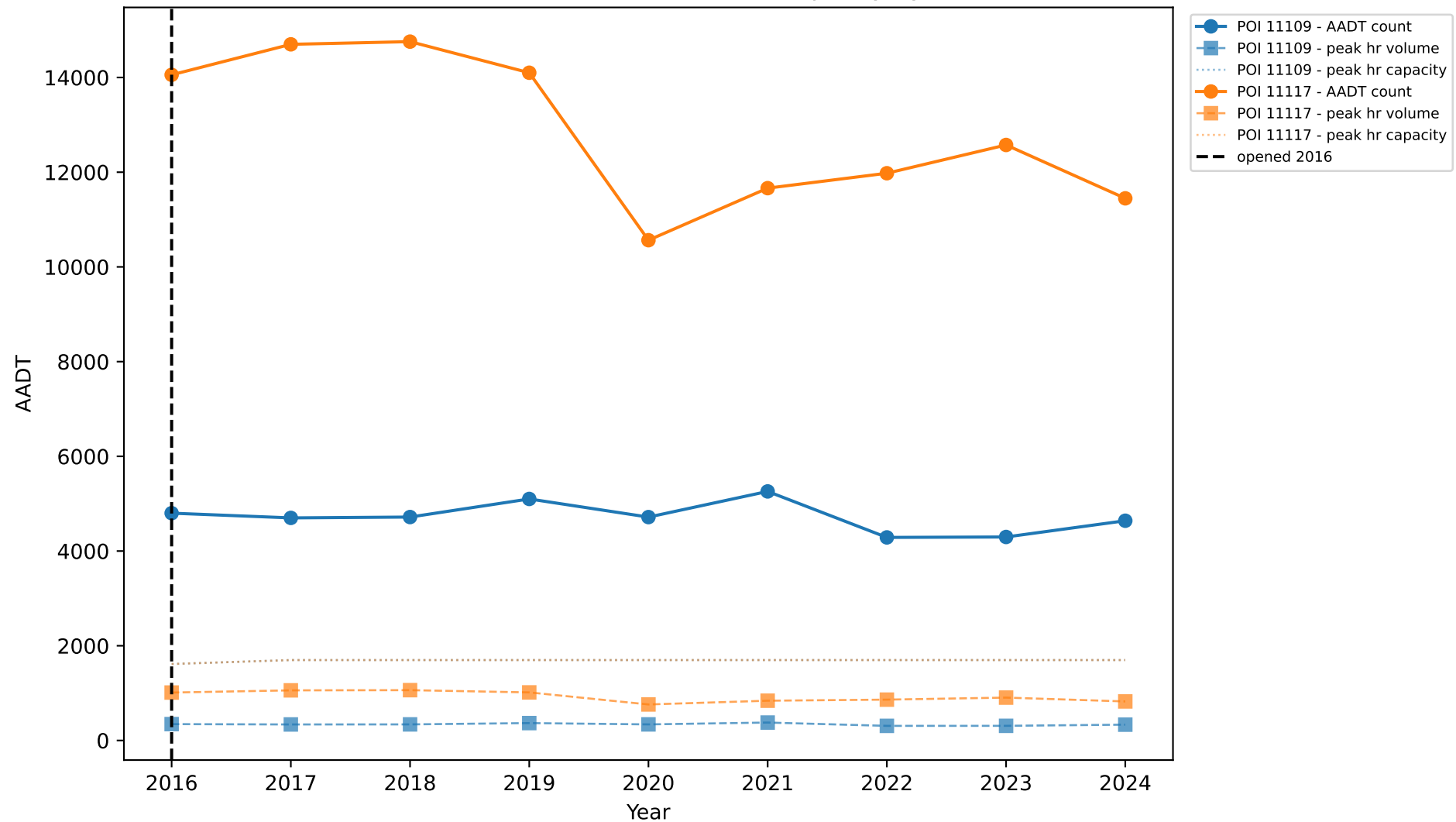
FM-1602: Traffic Counts, Peak Volume & Capacity by Station
