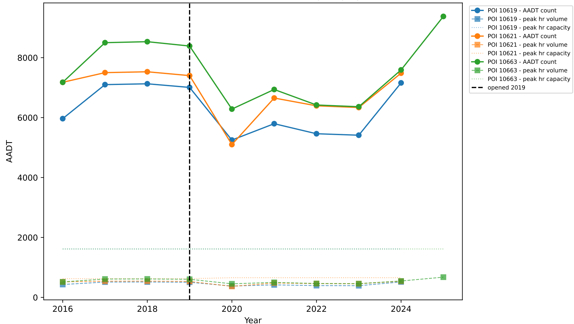
FM-1604: Traffic Counts, Peak Volume & Capacity by Station
