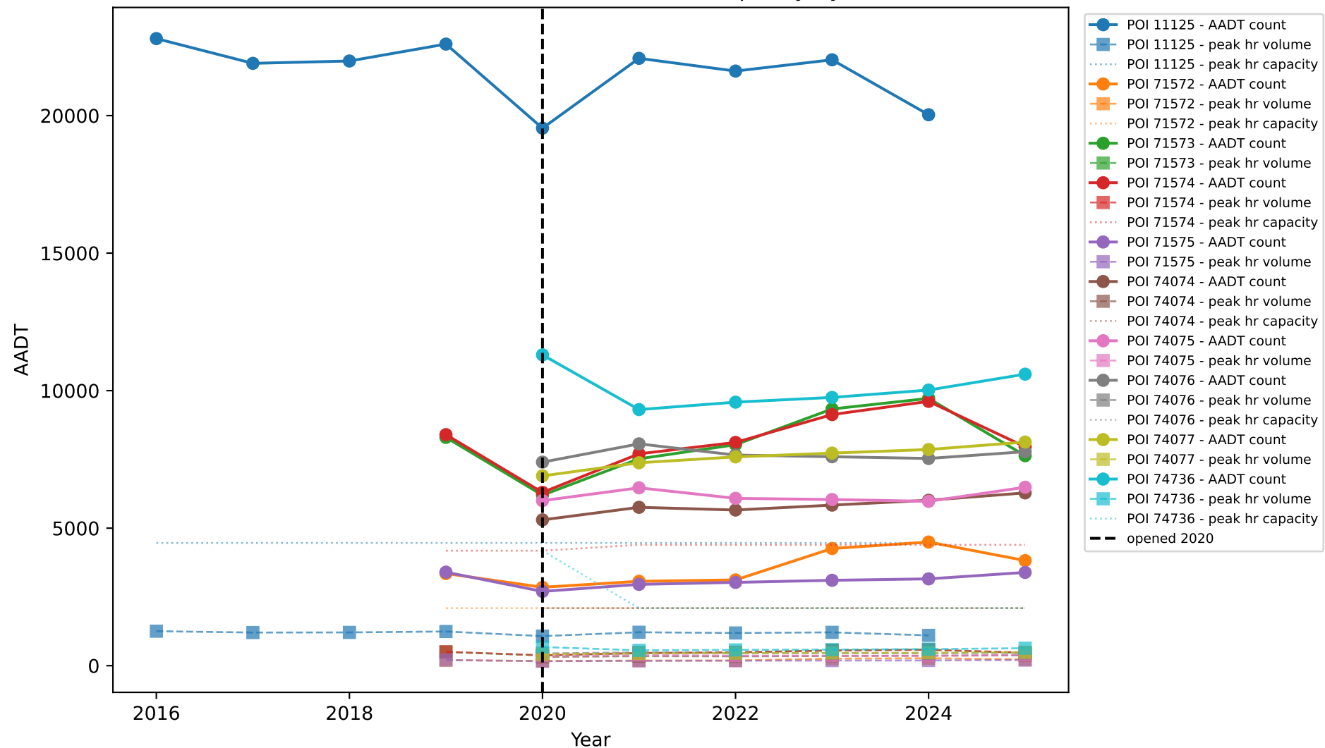
FM-1605: Traffic Counts, Peak Volume & Capacity by Station
