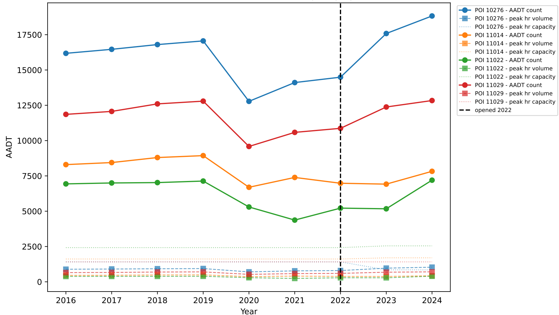
FM-1702: Traffic Counts, Peak Volume & Capacity by Station
