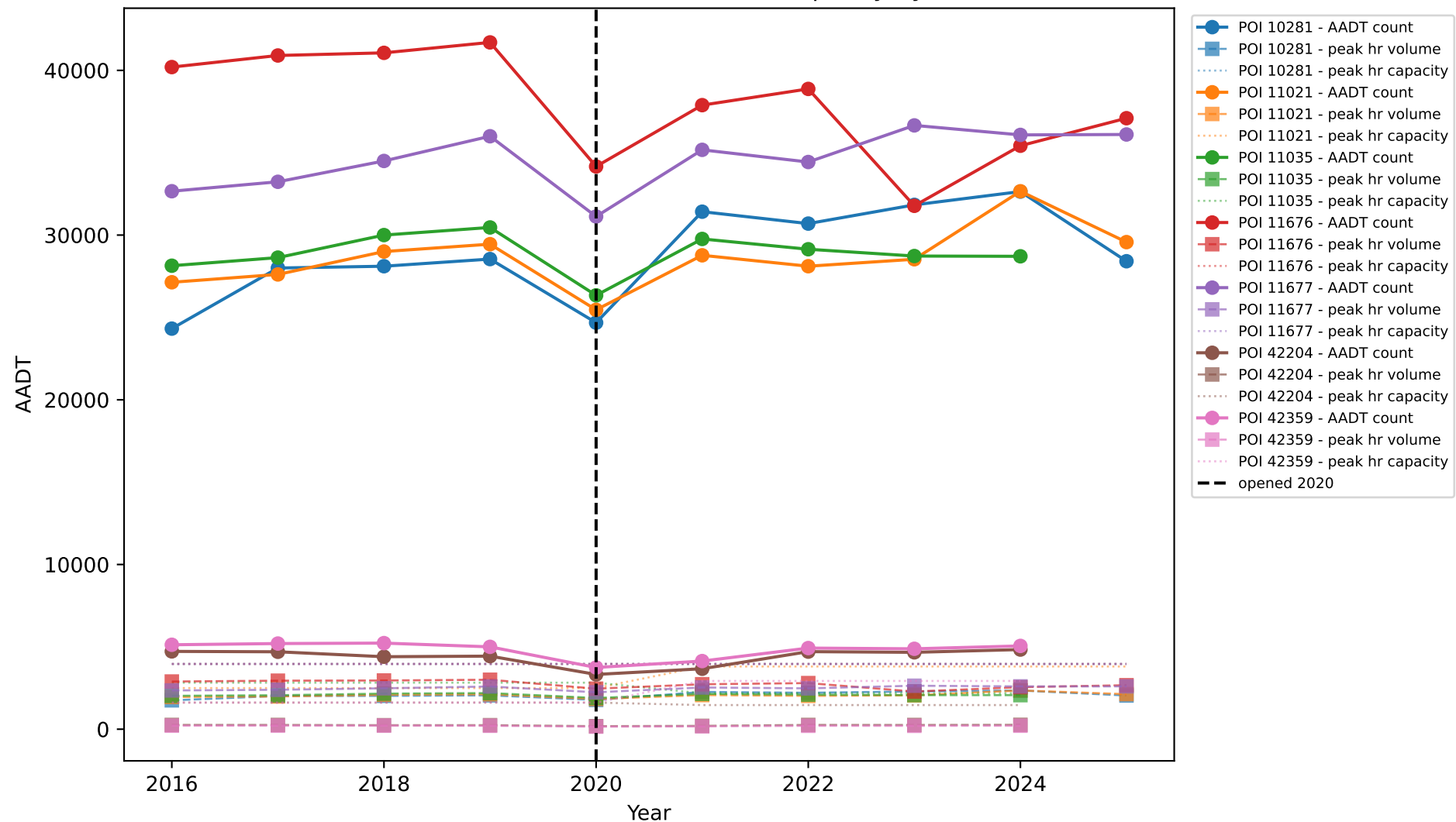
FM-1703: Traffic Counts, Peak Volume & Capacity by Station
