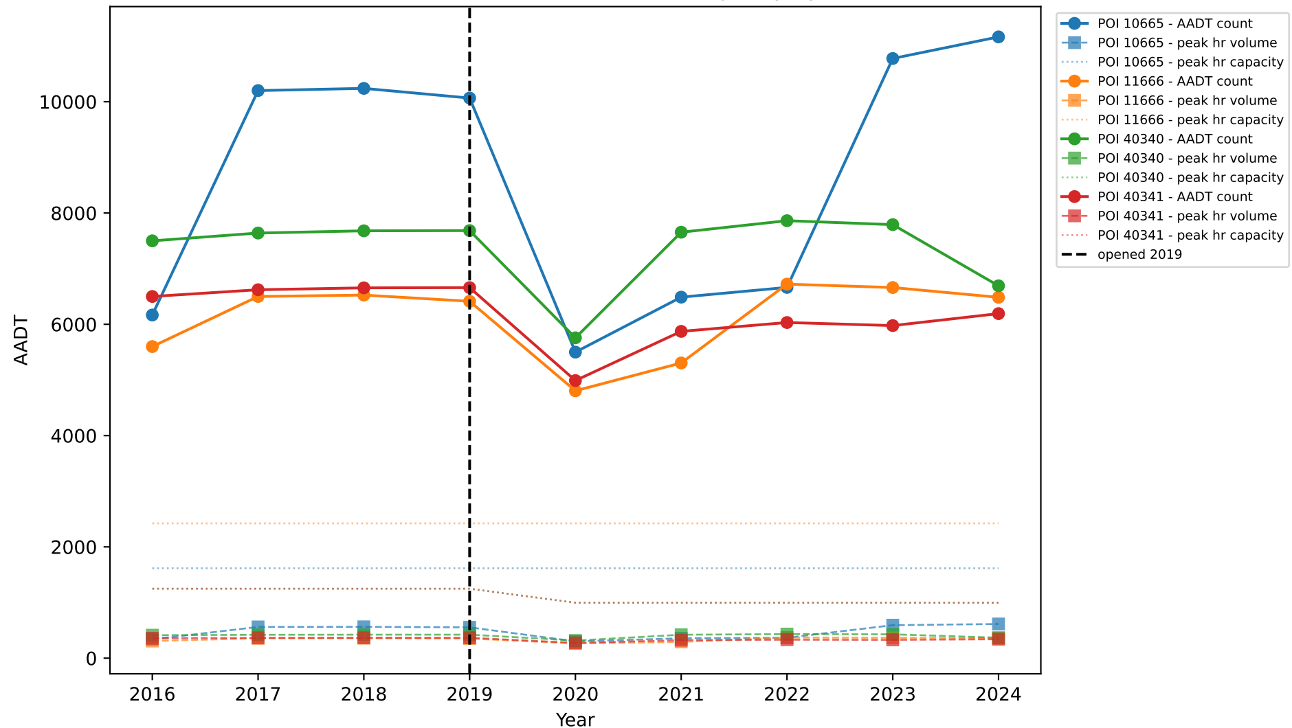
FM-1704: Traffic Counts, Peak Volume & Capacity by Station
