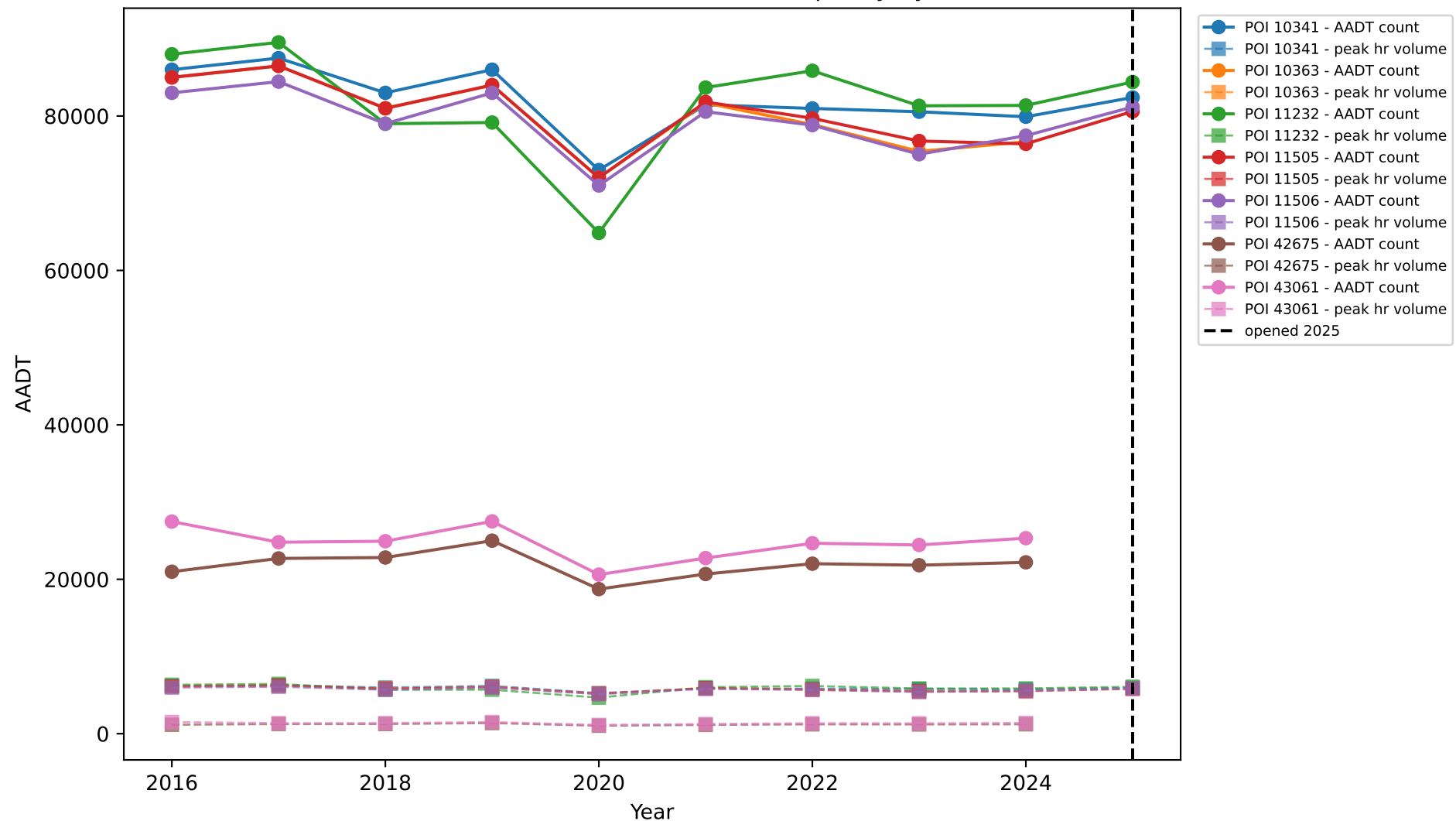
FM-1803: Traffic Counts, Peak Volume & Capacity by Station
