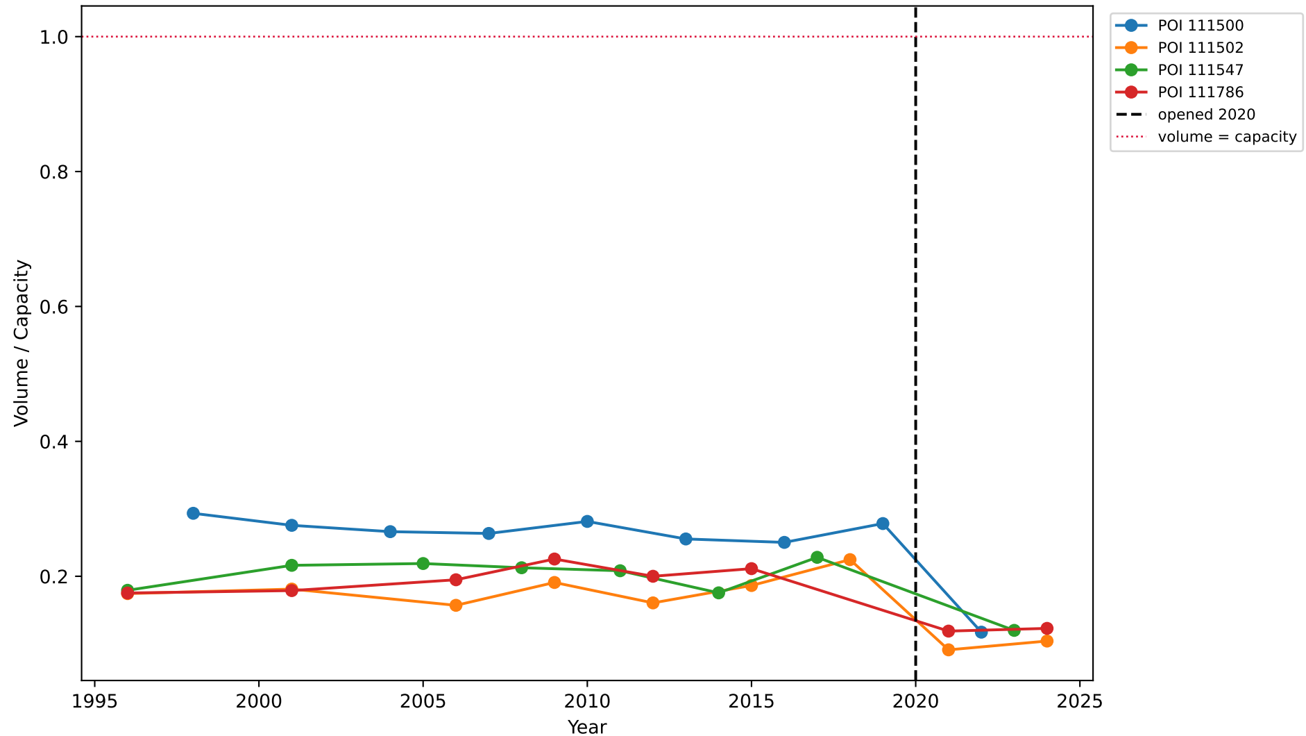
1-180.11: Volume-to-Capacity Ratio by Station
