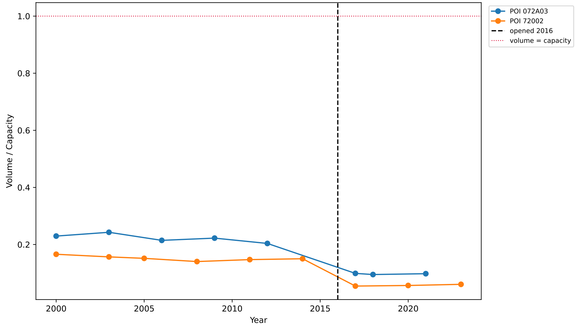
1-307.01: Volume-to-Capacity Ratio by Station
