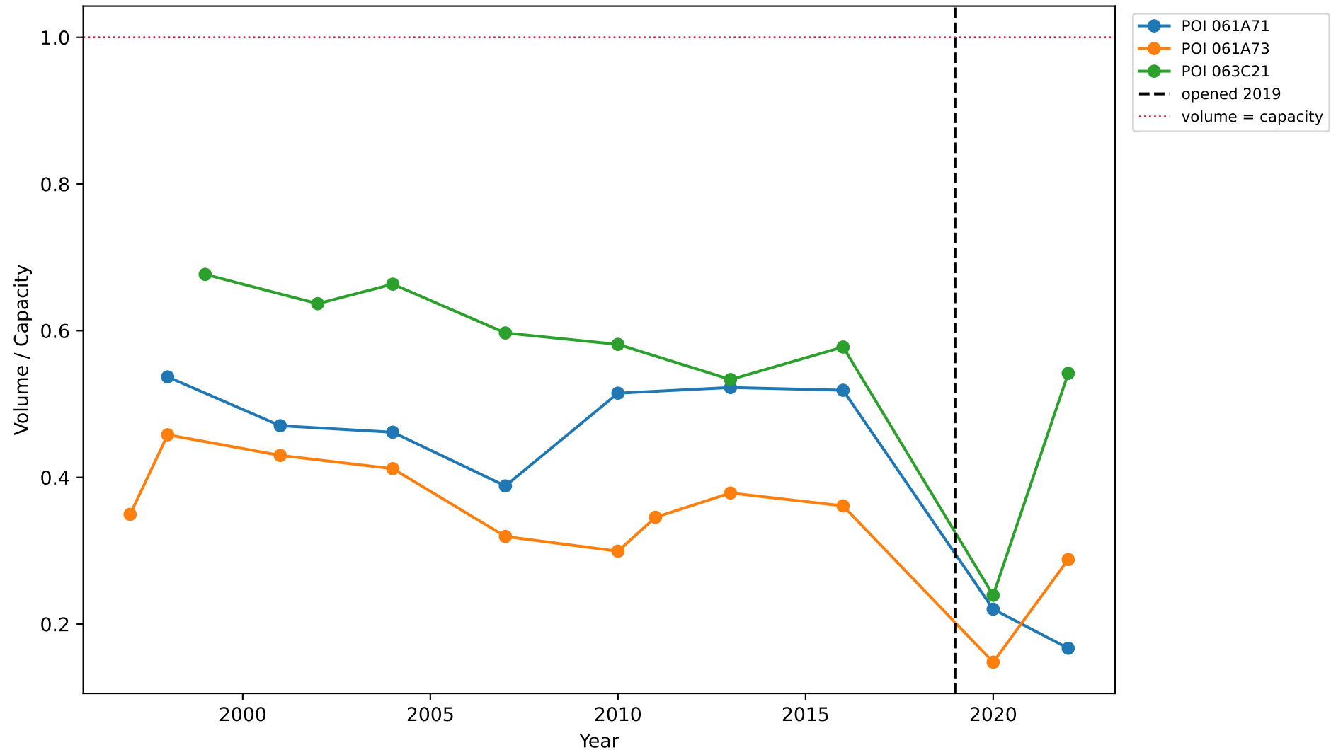
11-188.00: Volume-to-Capacity Ratio by Station
