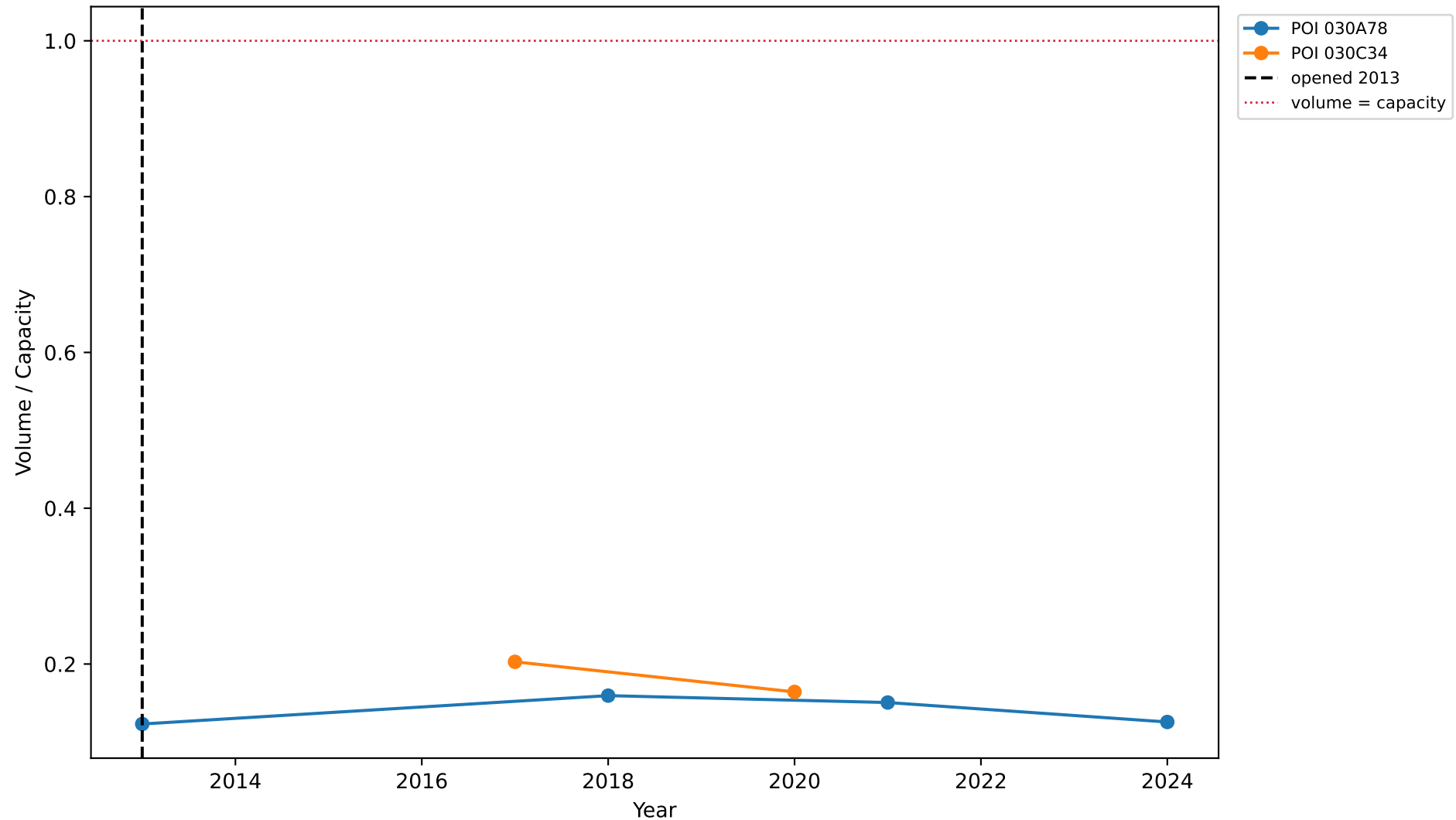
2-221.00: Volume-to-Capacity Ratio by Station
