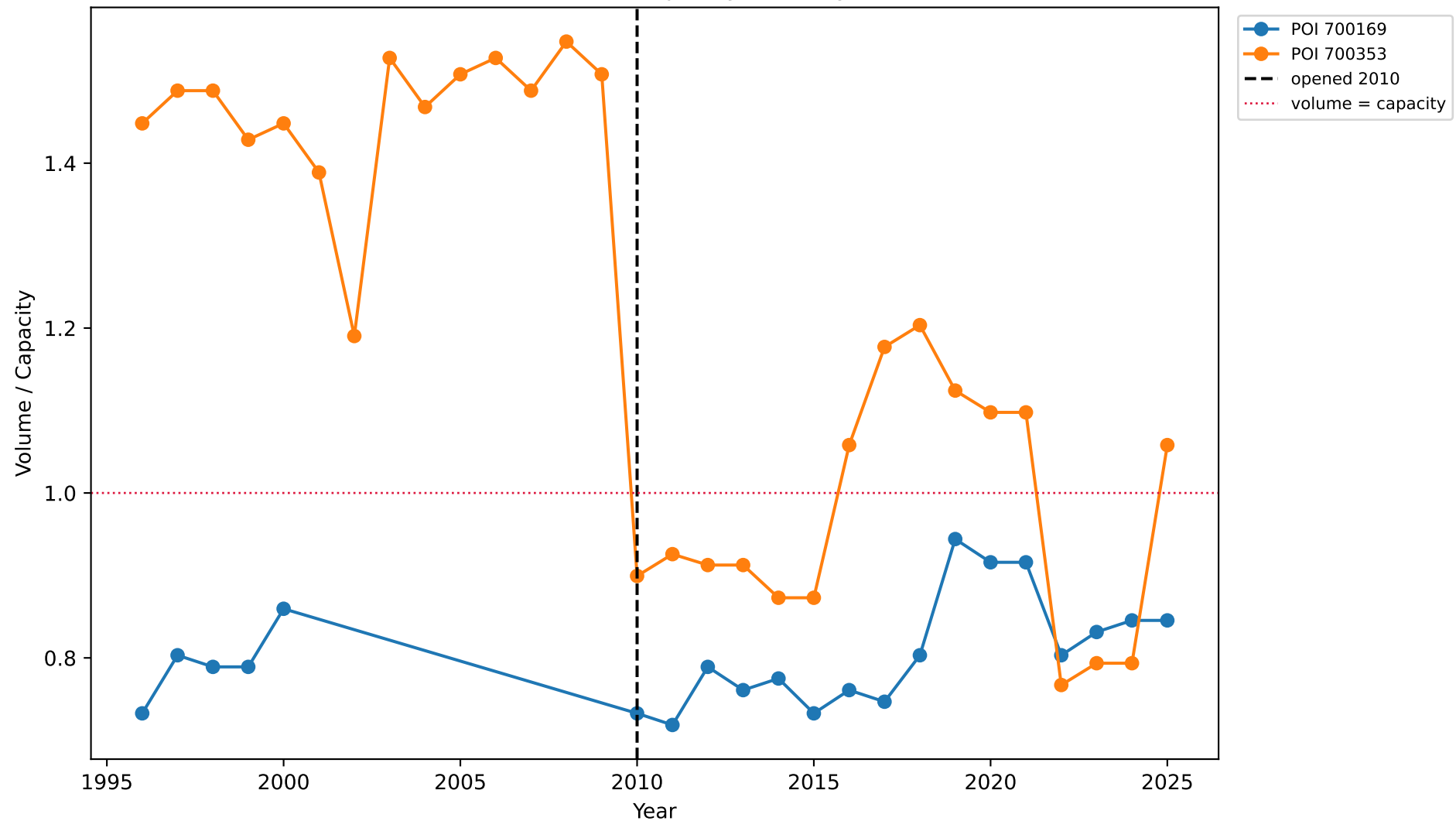
237576-1: Volume-to-Capacity Ratio by Station
