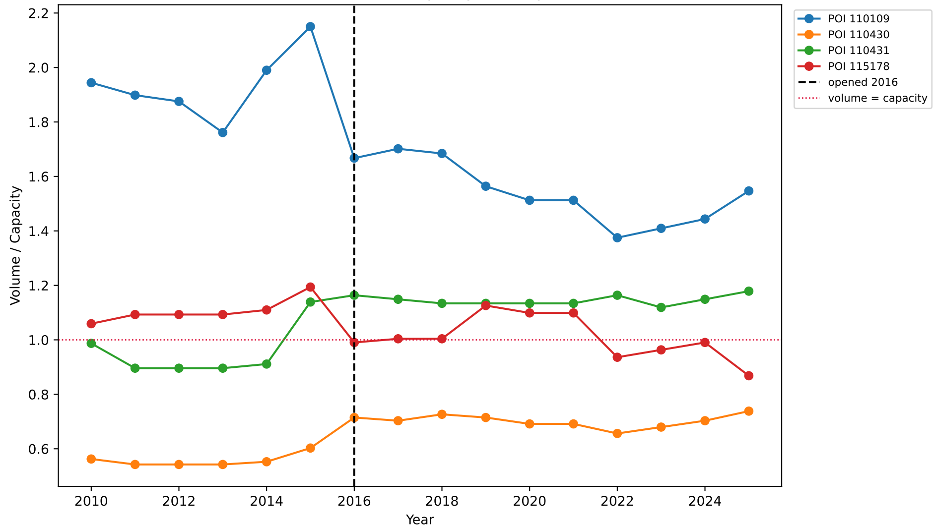
238395-4: Volume-to-Capacity Ratio by Station
