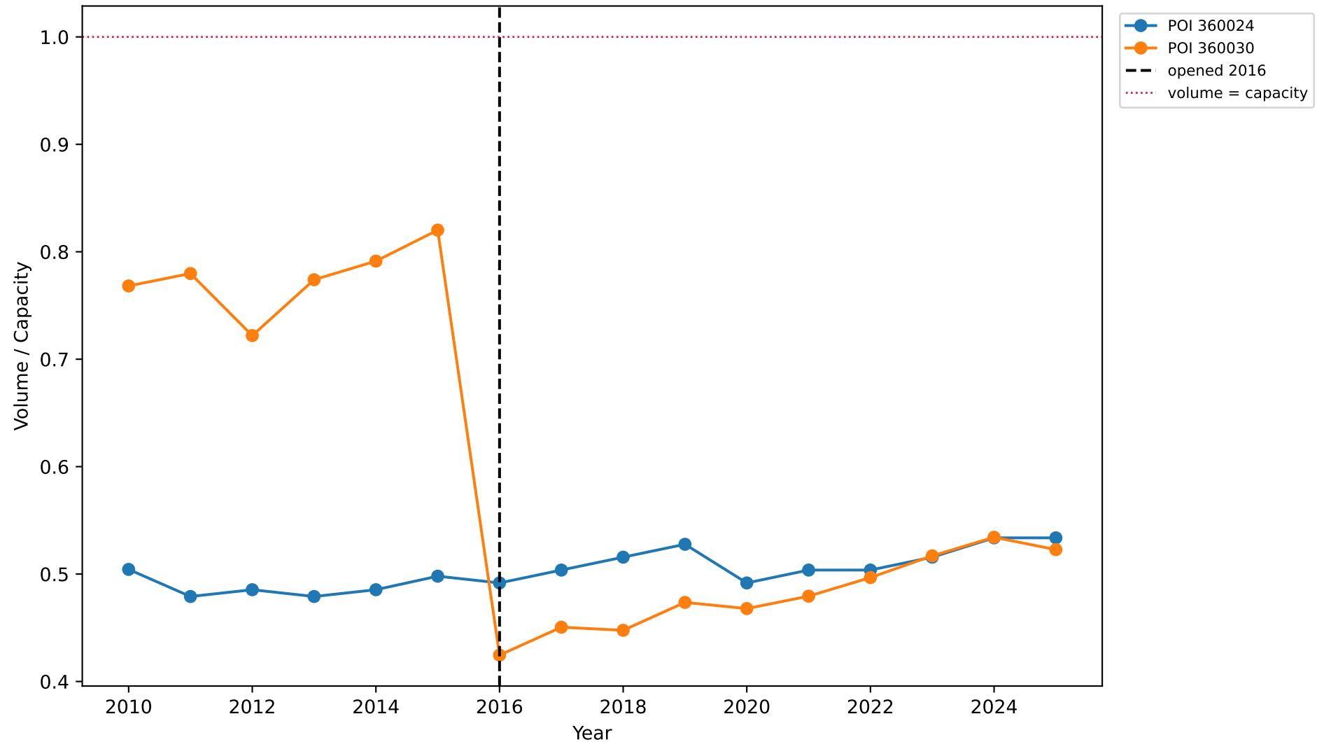
238720-1: Volume-to-Capacity Ratio by Station
