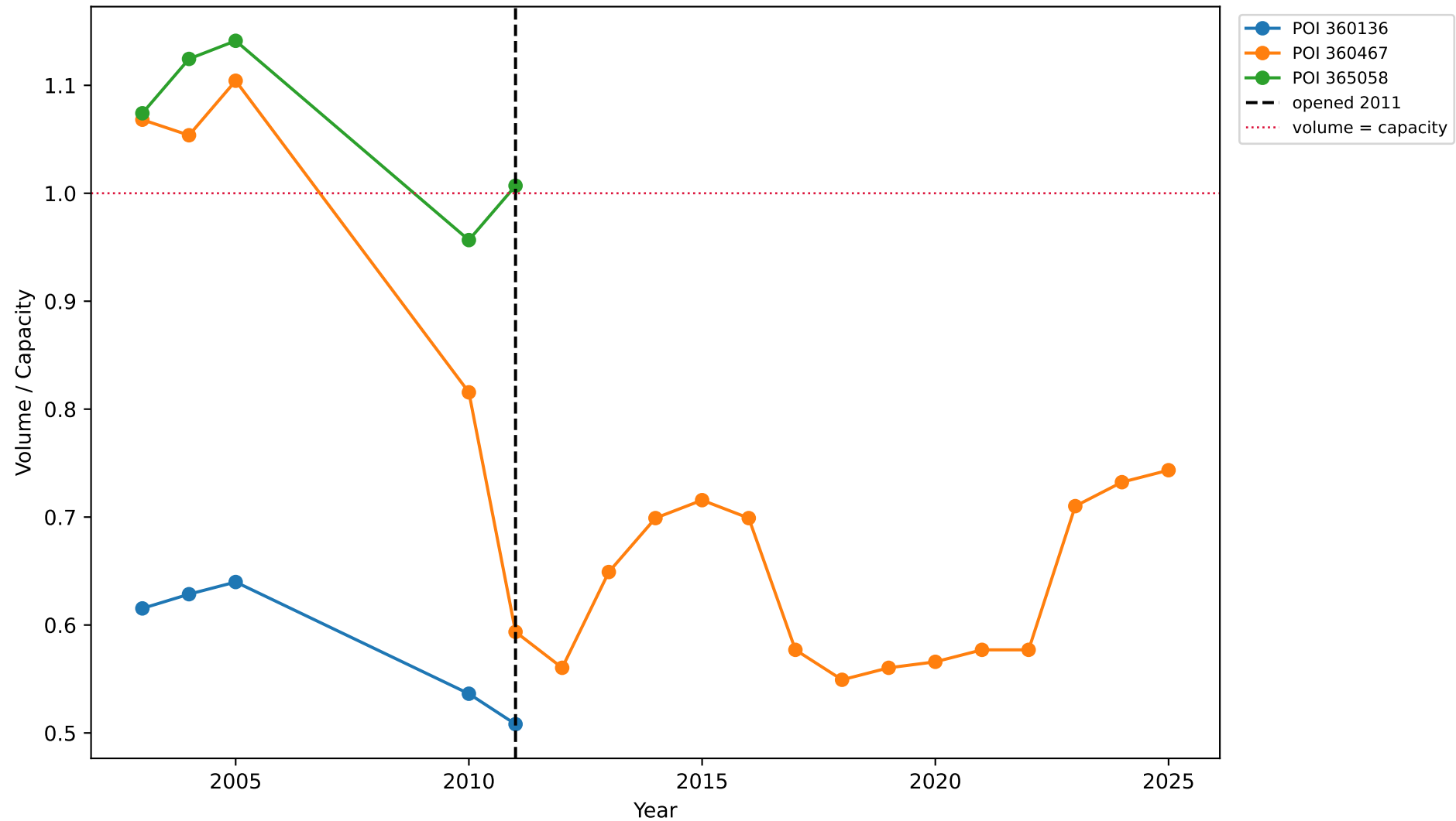
238753-1A: Volume-to-Capacity Ratio by Station
