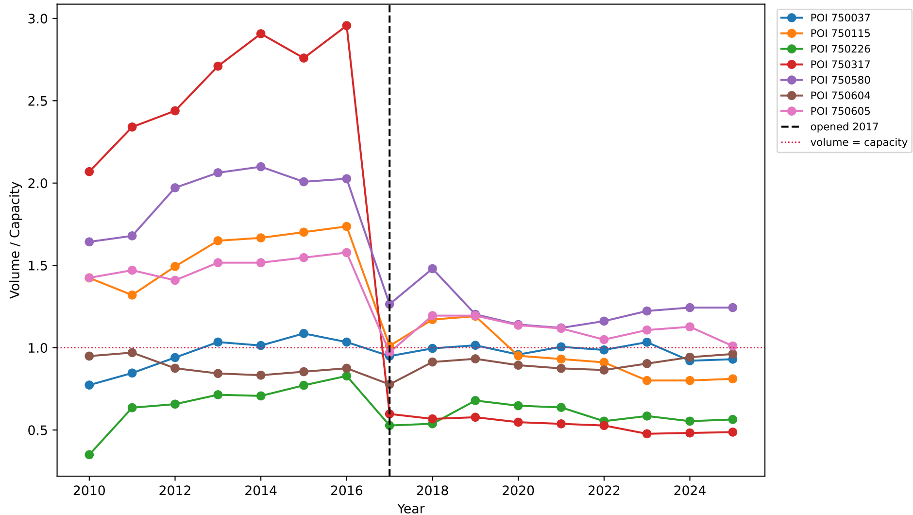
239203-2: Volume-to-Capacity Ratio by Station
