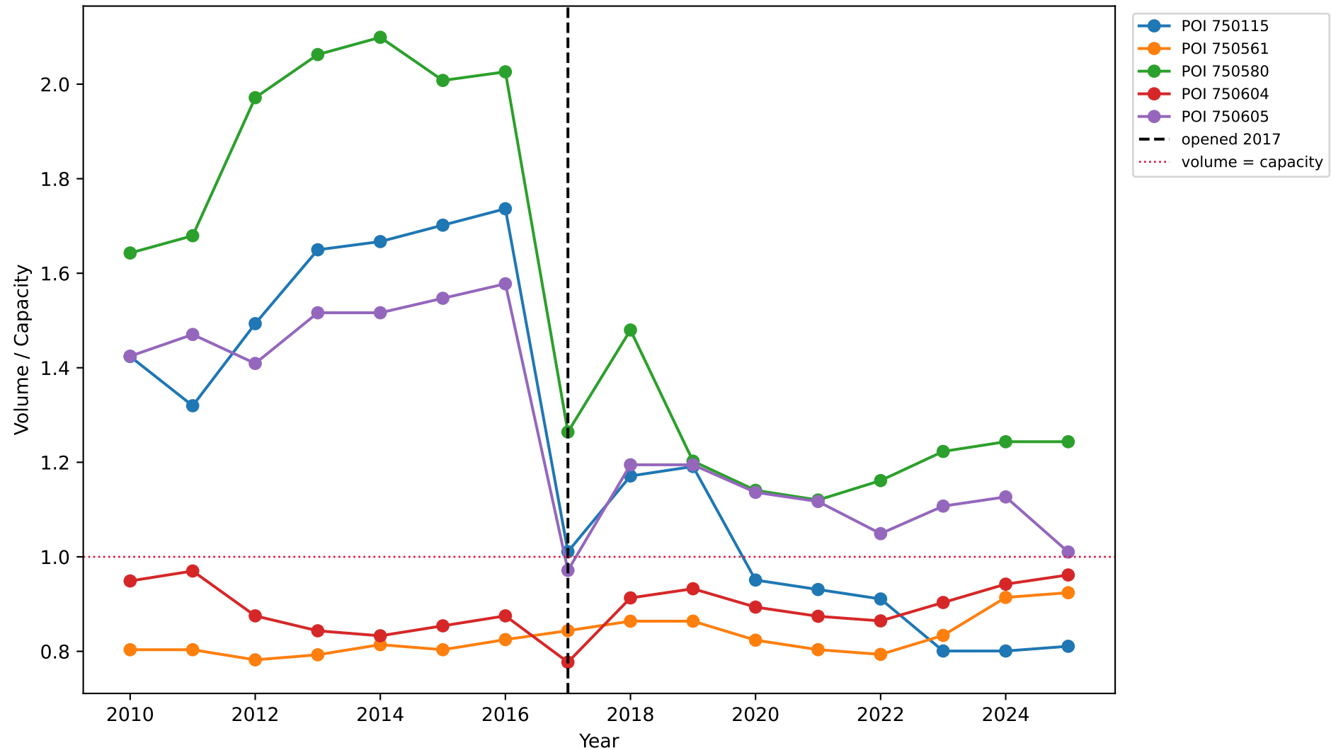
239203-4: Volume-to-Capacity Ratio by Station
