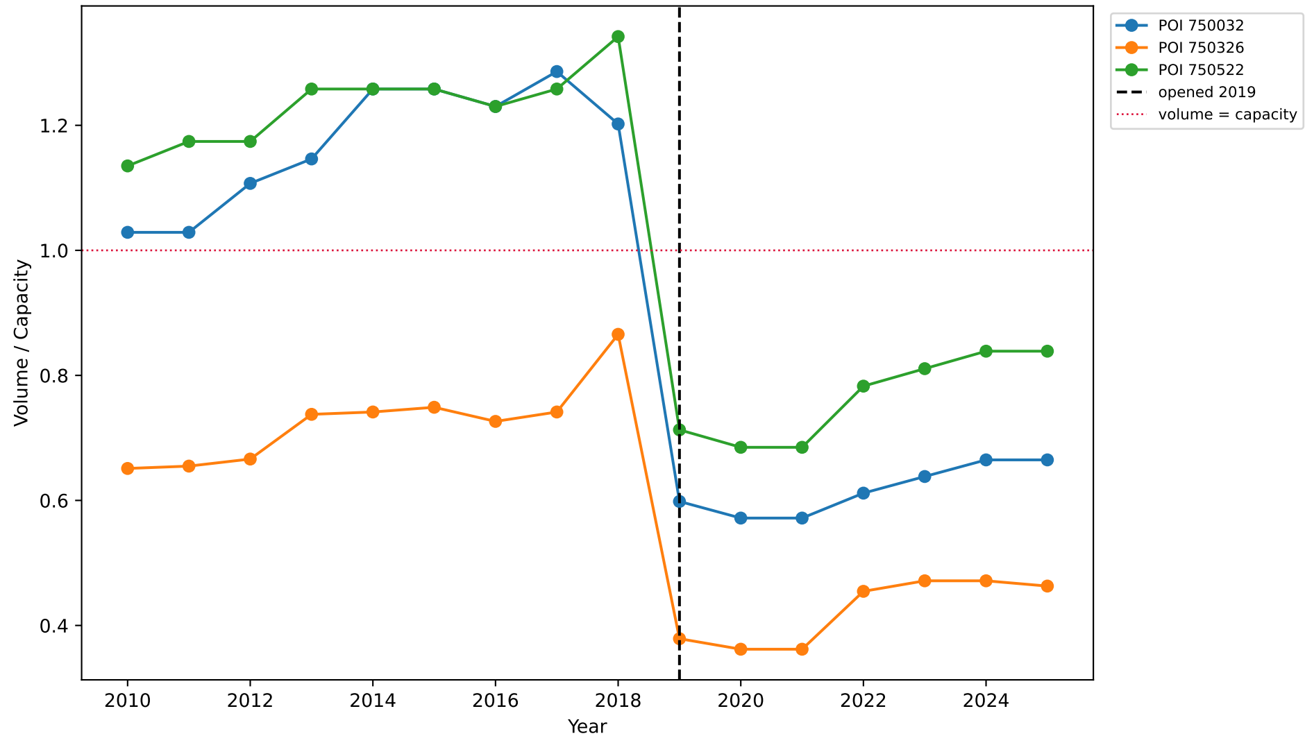
239266-3: Volume-to-Capacity Ratio by Station
