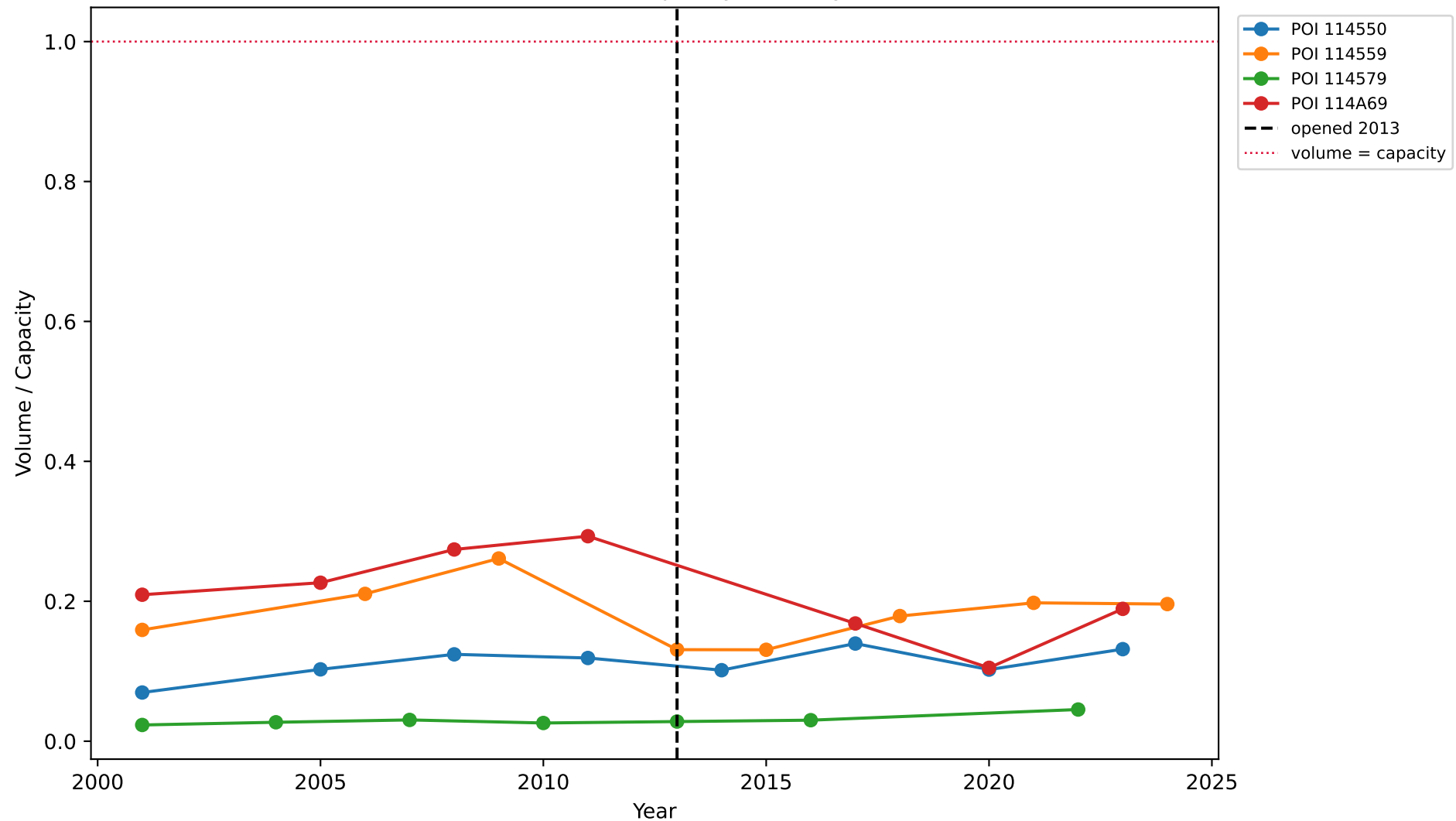
3-102.10: Volume-to-Capacity Ratio by Station
