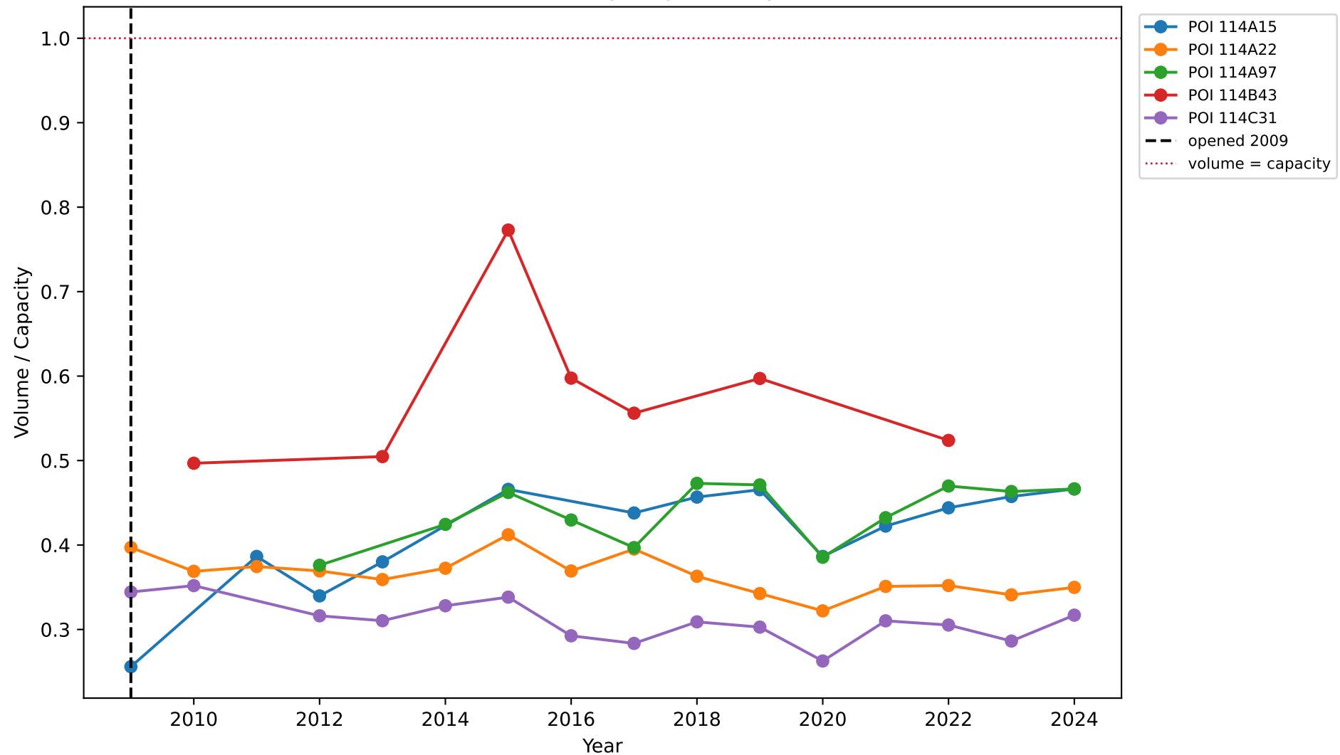
3-312.00: Volume-to-Capacity Ratio by Station
