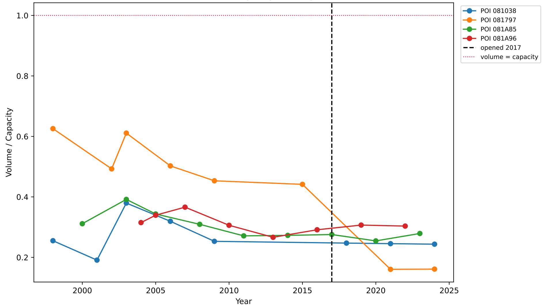
9-169.00: Volume-to-Capacity Ratio by Station
