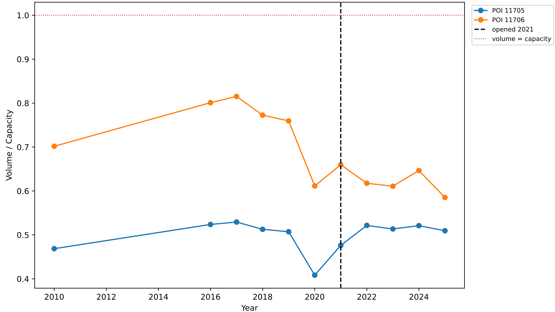
FM-0804: Volume-to-Capacity Ratio by Station
