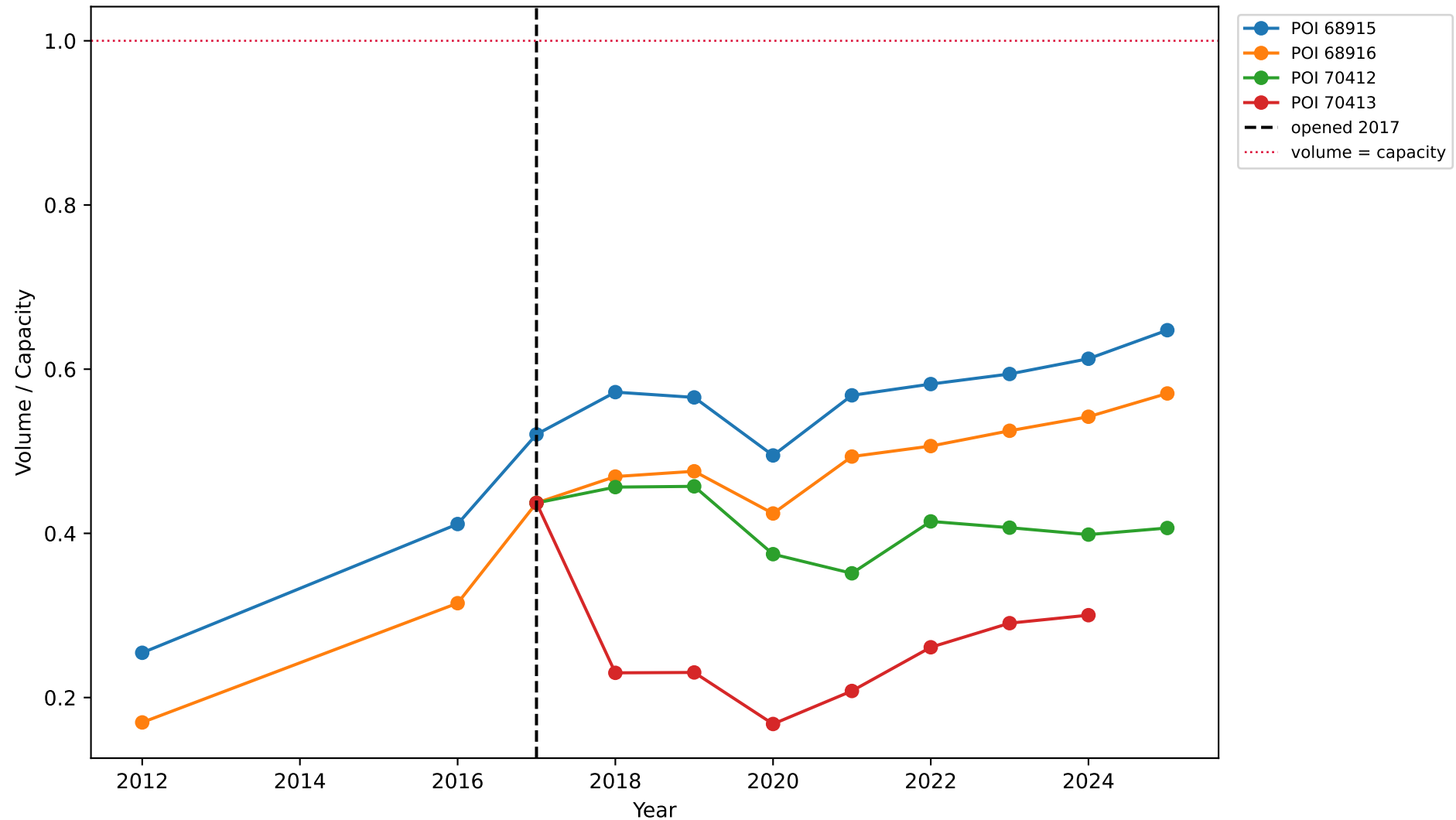
FM-0902: Volume-to-Capacity Ratio by Station
