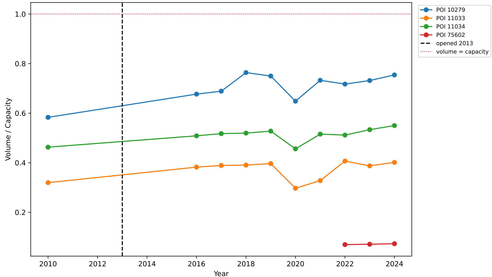
FM-0915: Volume-to-Capacity Ratio by Station
