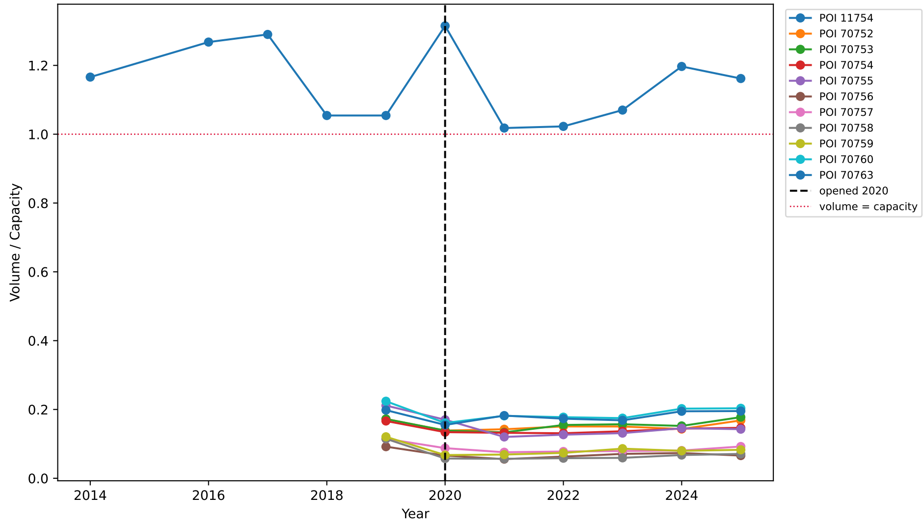
FM-1314: Volume-to-Capacity Ratio by Station
