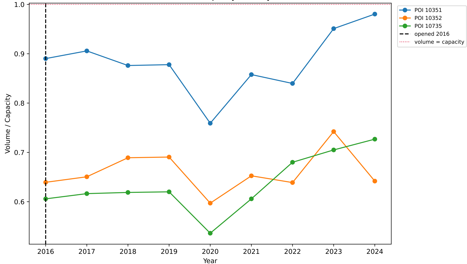
FM-1403: Volume-to-Capacity Ratio by Station
