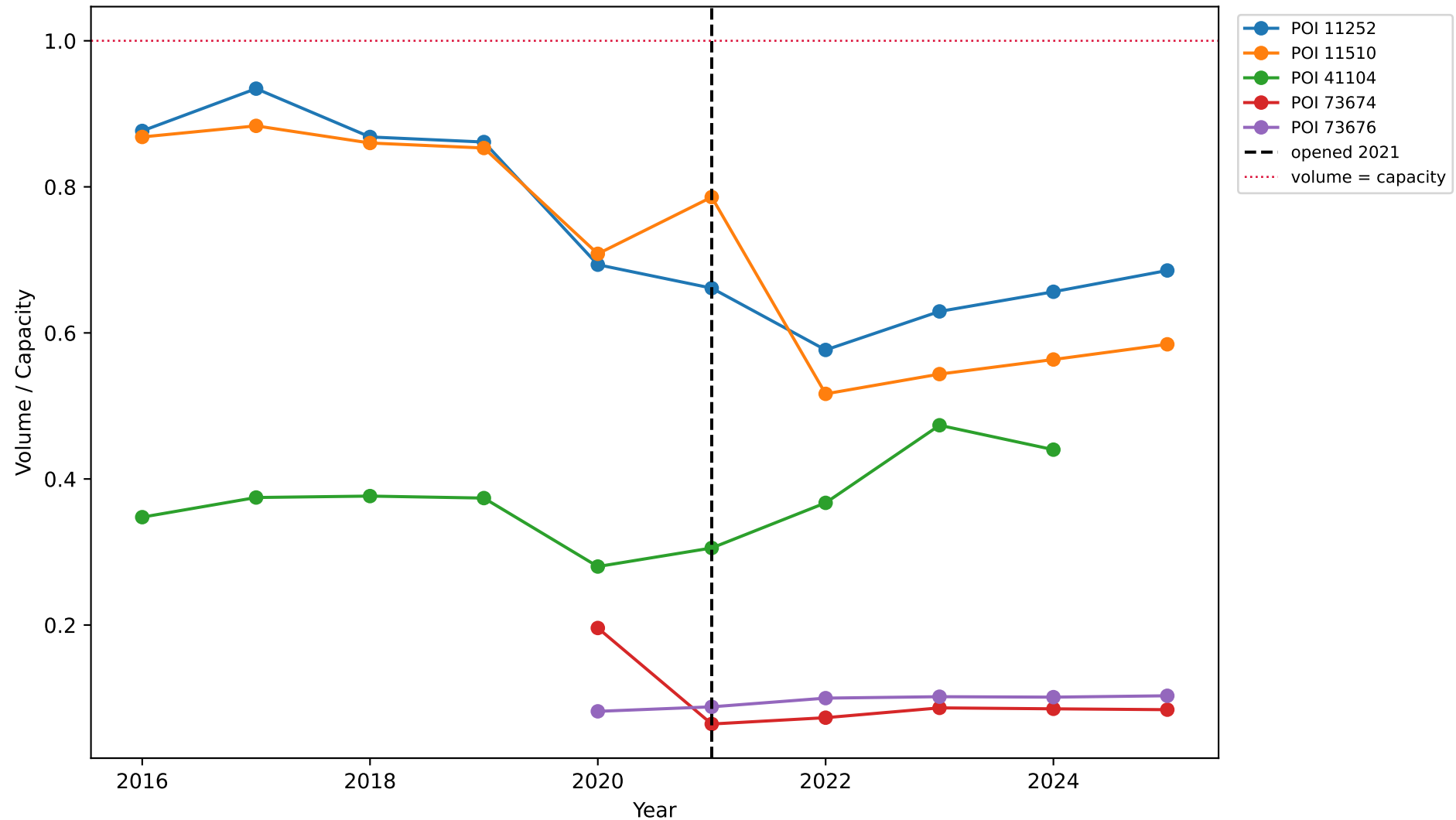
FM-1405: Volume-to-Capacity Ratio by Station
