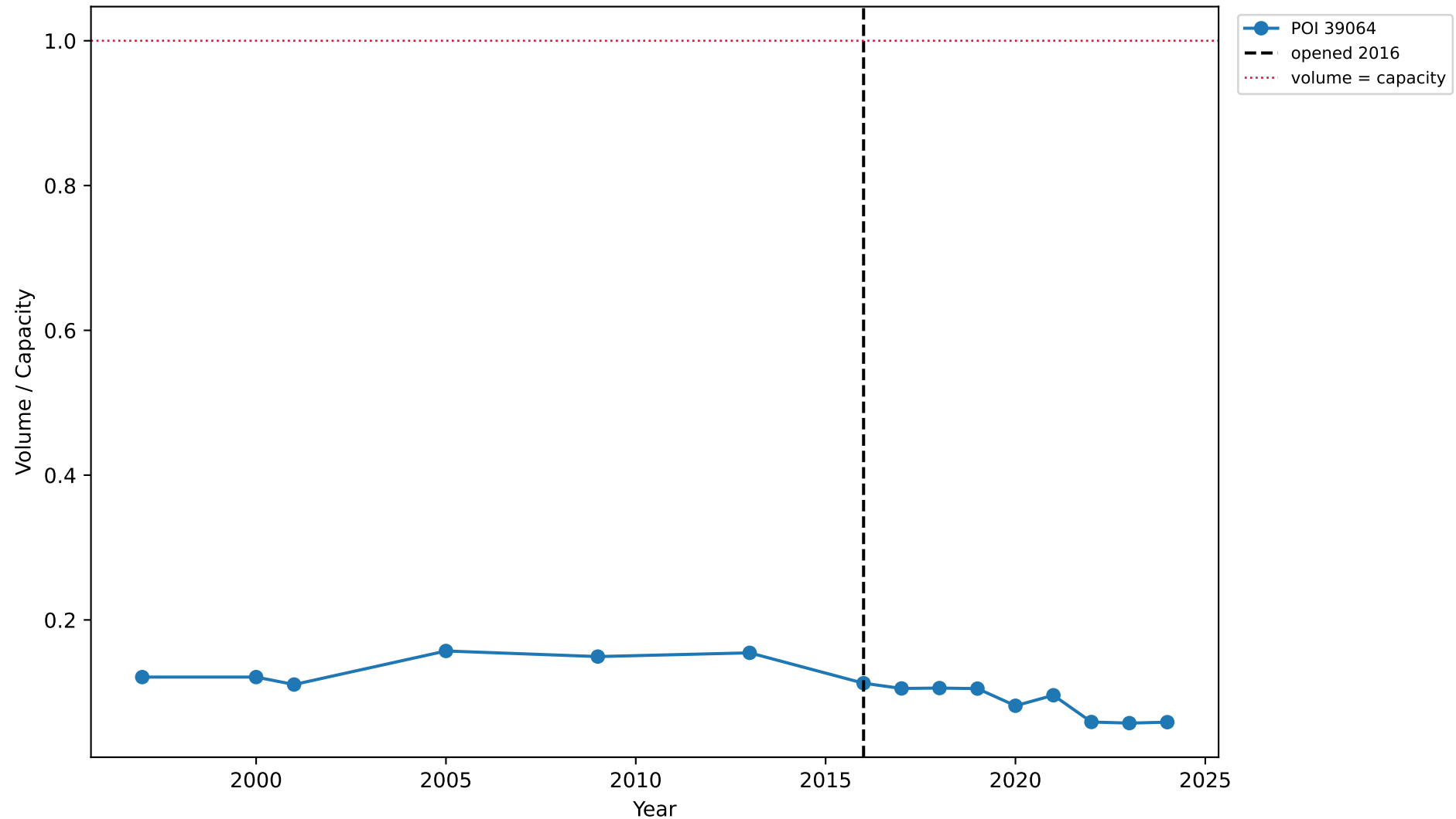
FM-1408: Volume-to-Capacity Ratio by Station
