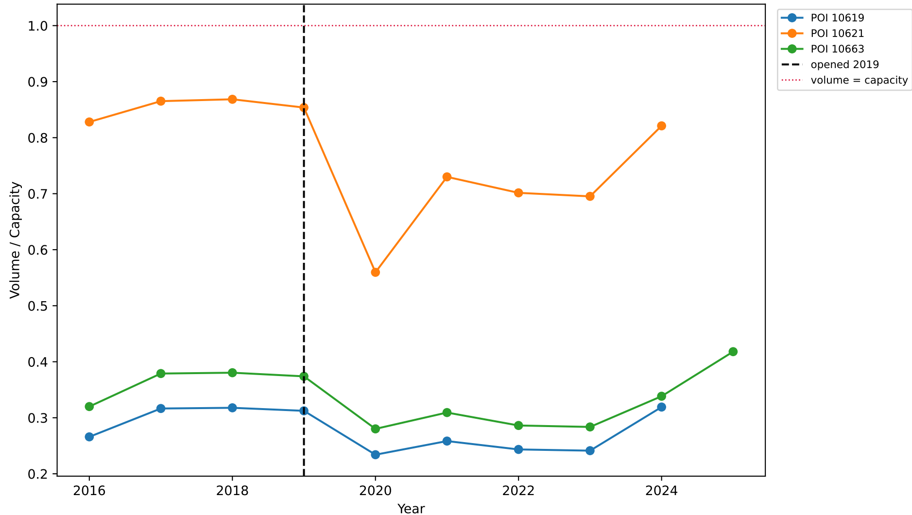
FM-1604: Volume-to-Capacity Ratio by Station
