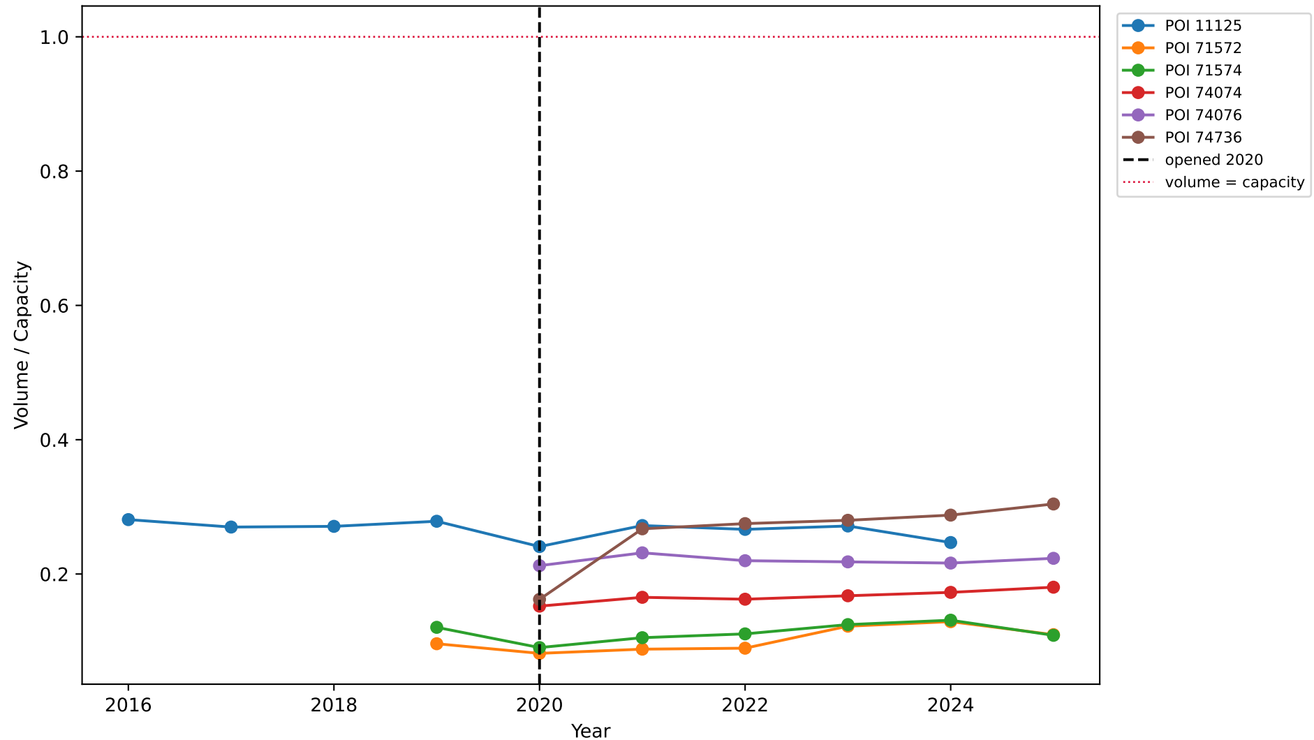
FM-1605: Volume-to-Capacity Ratio by Station
