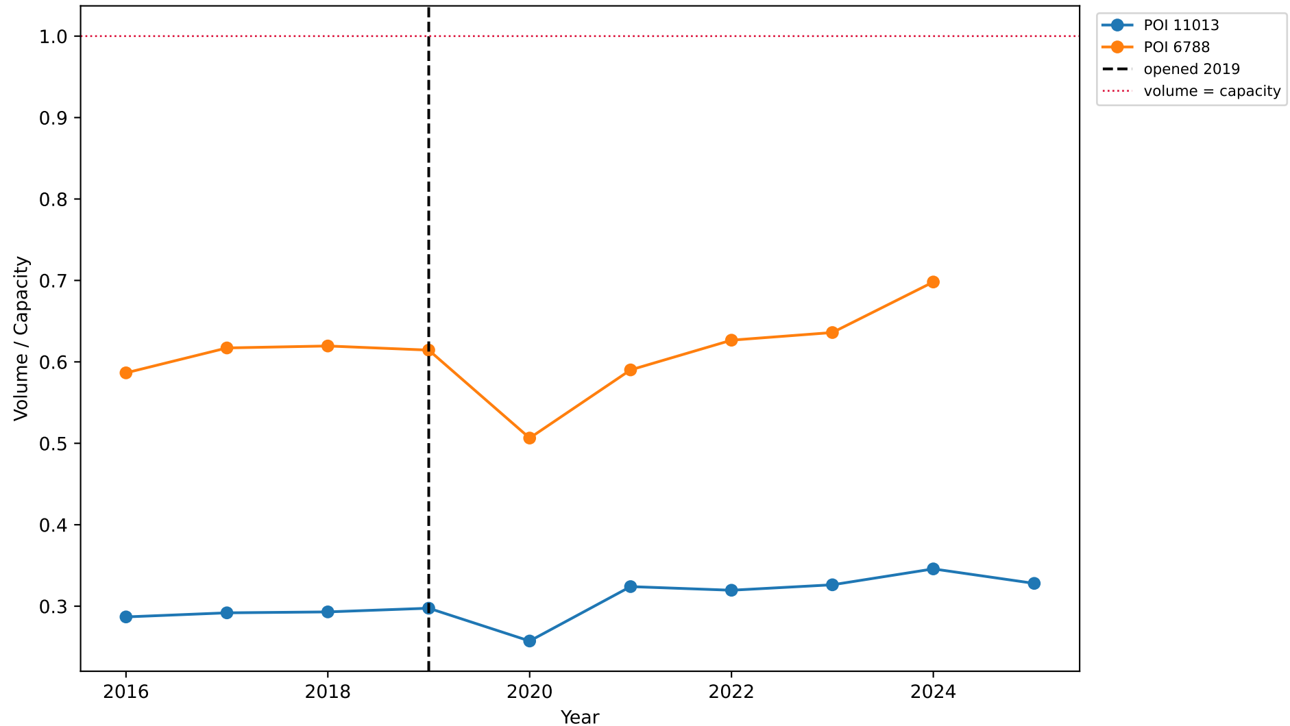
FM-1606: Volume-to-Capacity Ratio by Station
