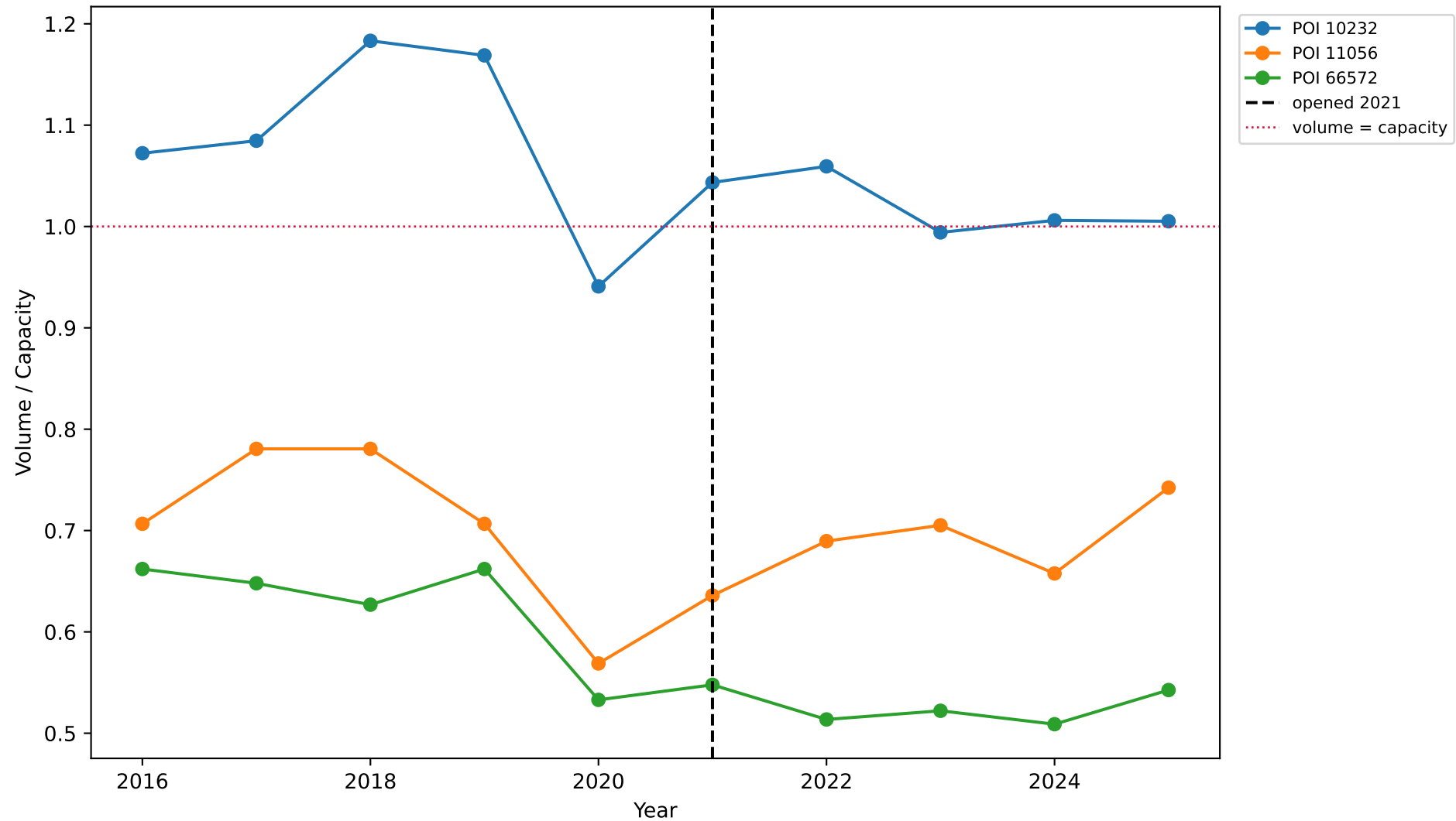
FM-1701: Volume-to-Capacity Ratio by Station
