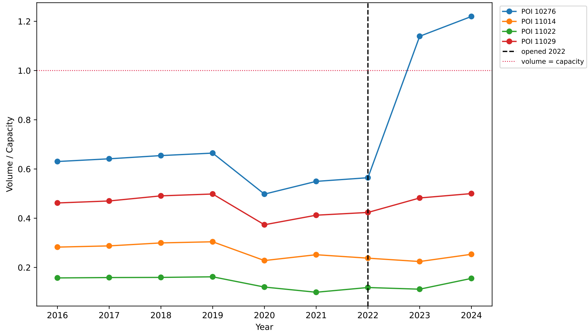
FM-1702: Volume-to-Capacity Ratio by Station
