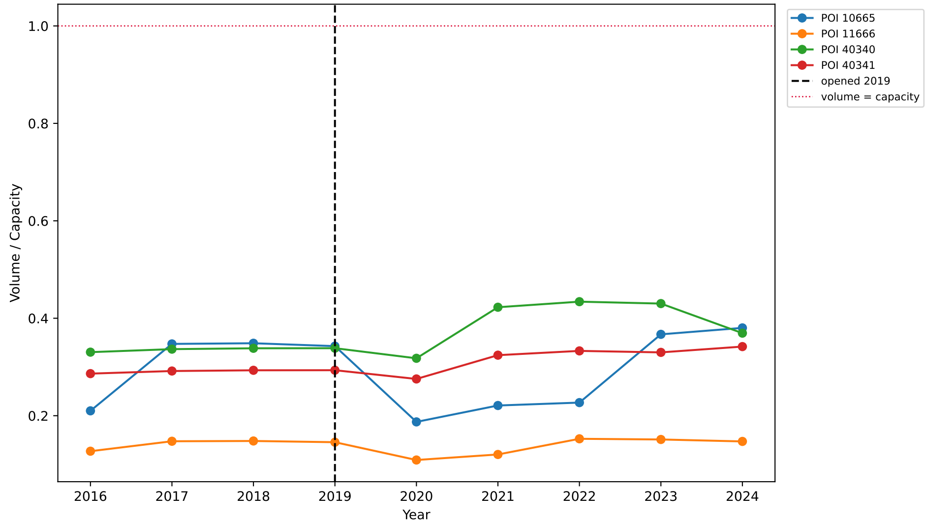
FM-1704: Volume-to-Capacity Ratio by Station
