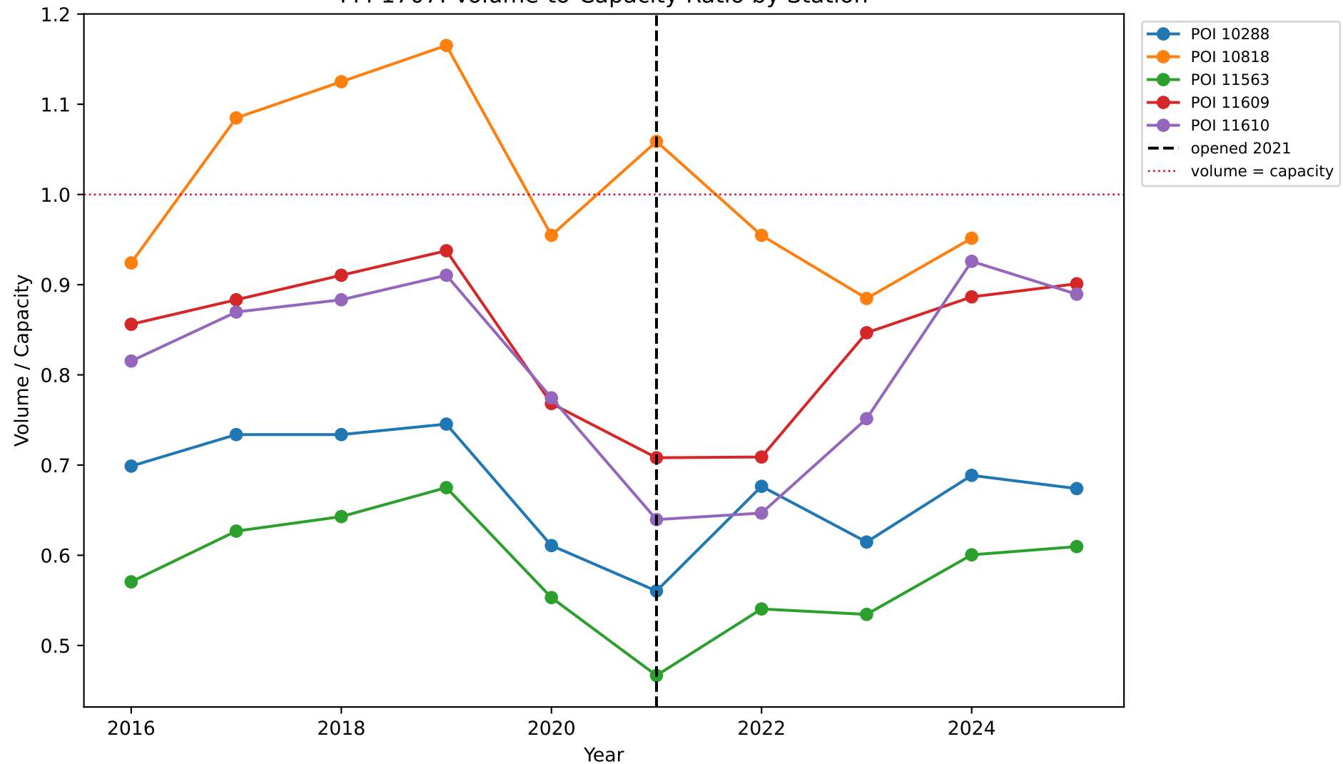
FM-1707: Volume-to-Capacity Ratio by Station
