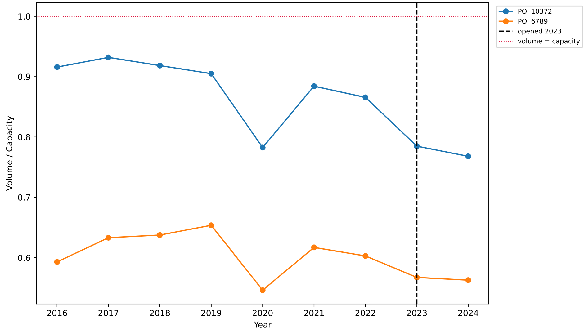
FM-1903: Volume-to-Capacity Ratio by Station
