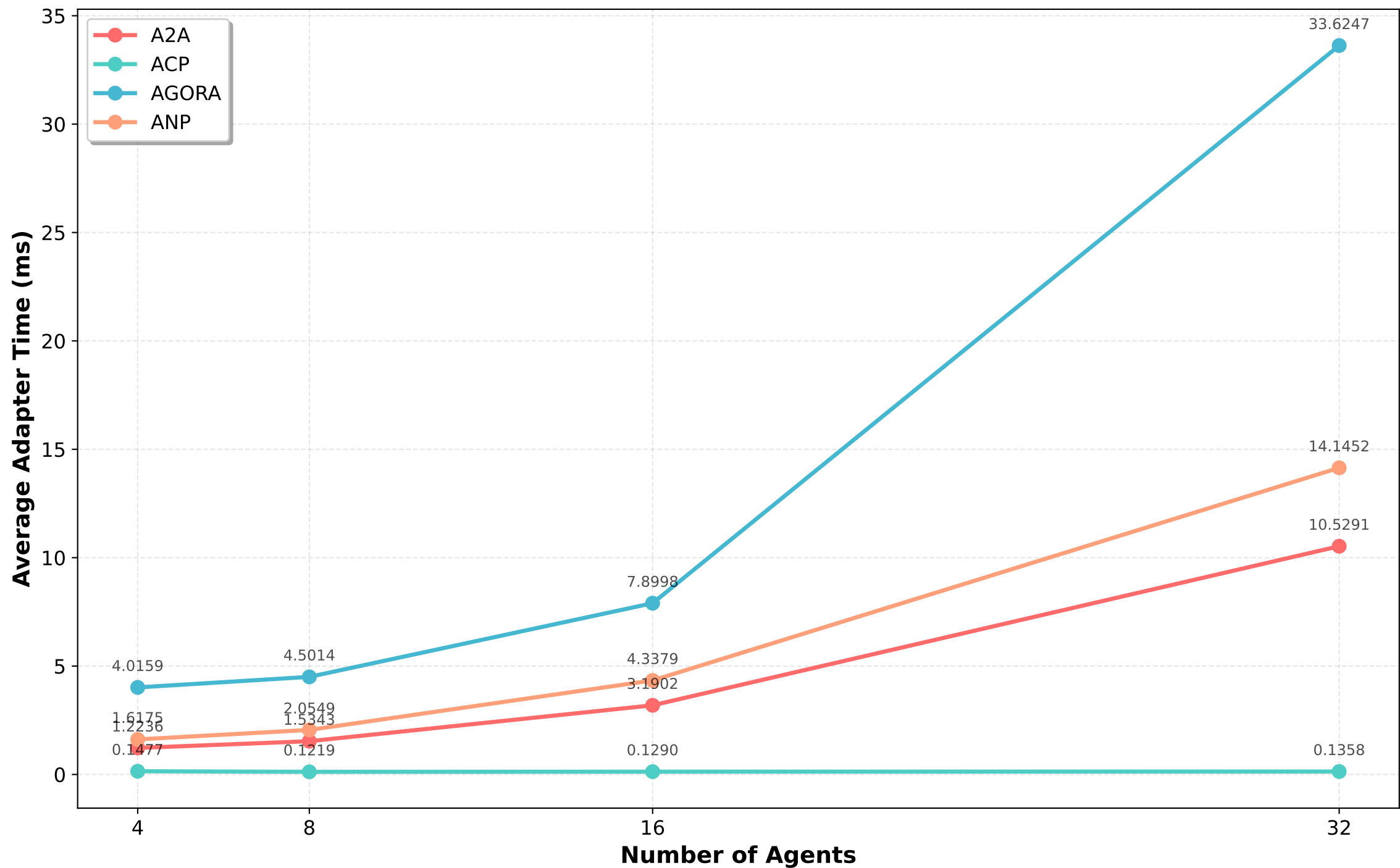
Adapter Performance vs Agent Count for Different Protocols
