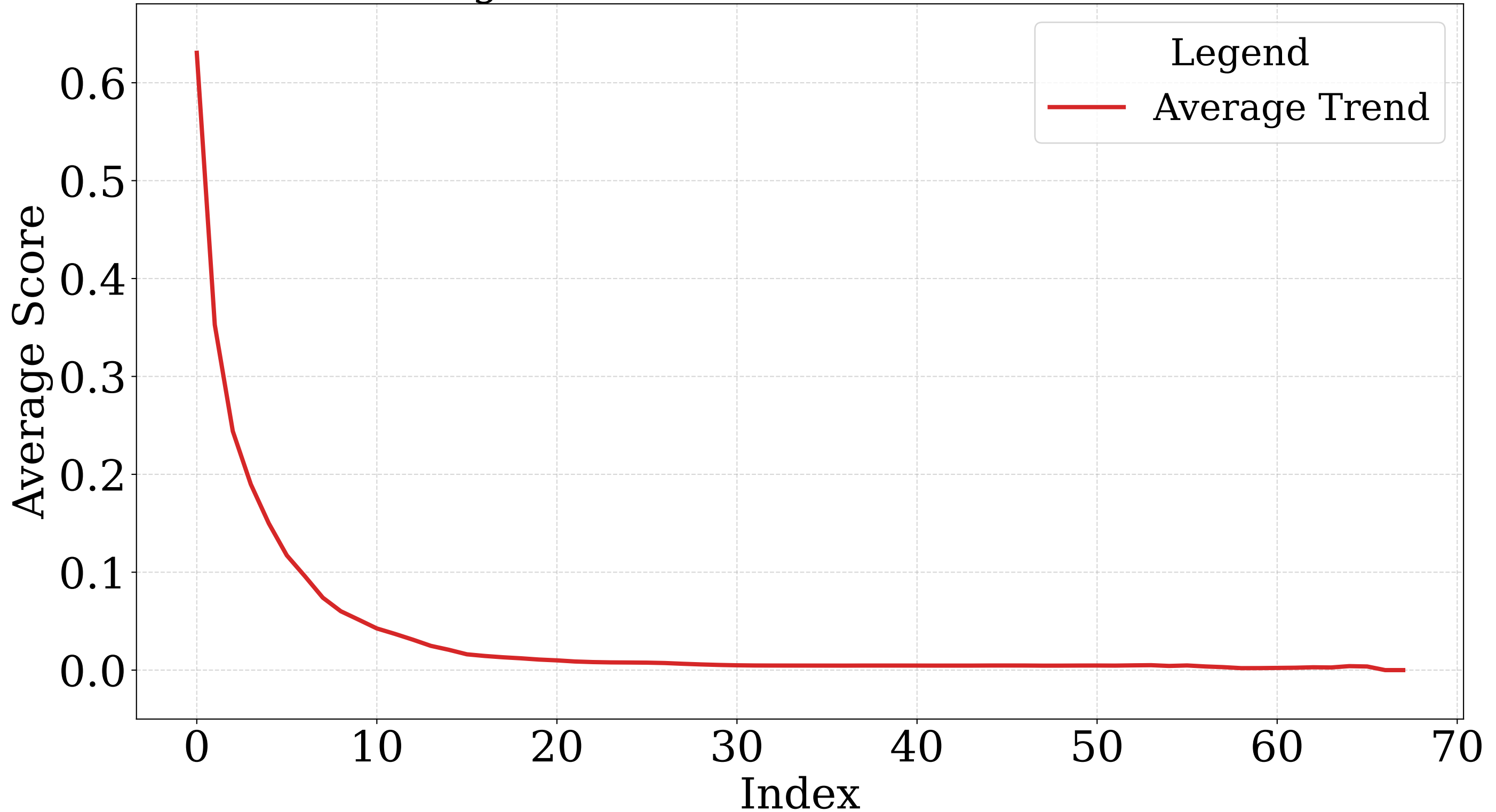
Average Value Trend Across Distributions
