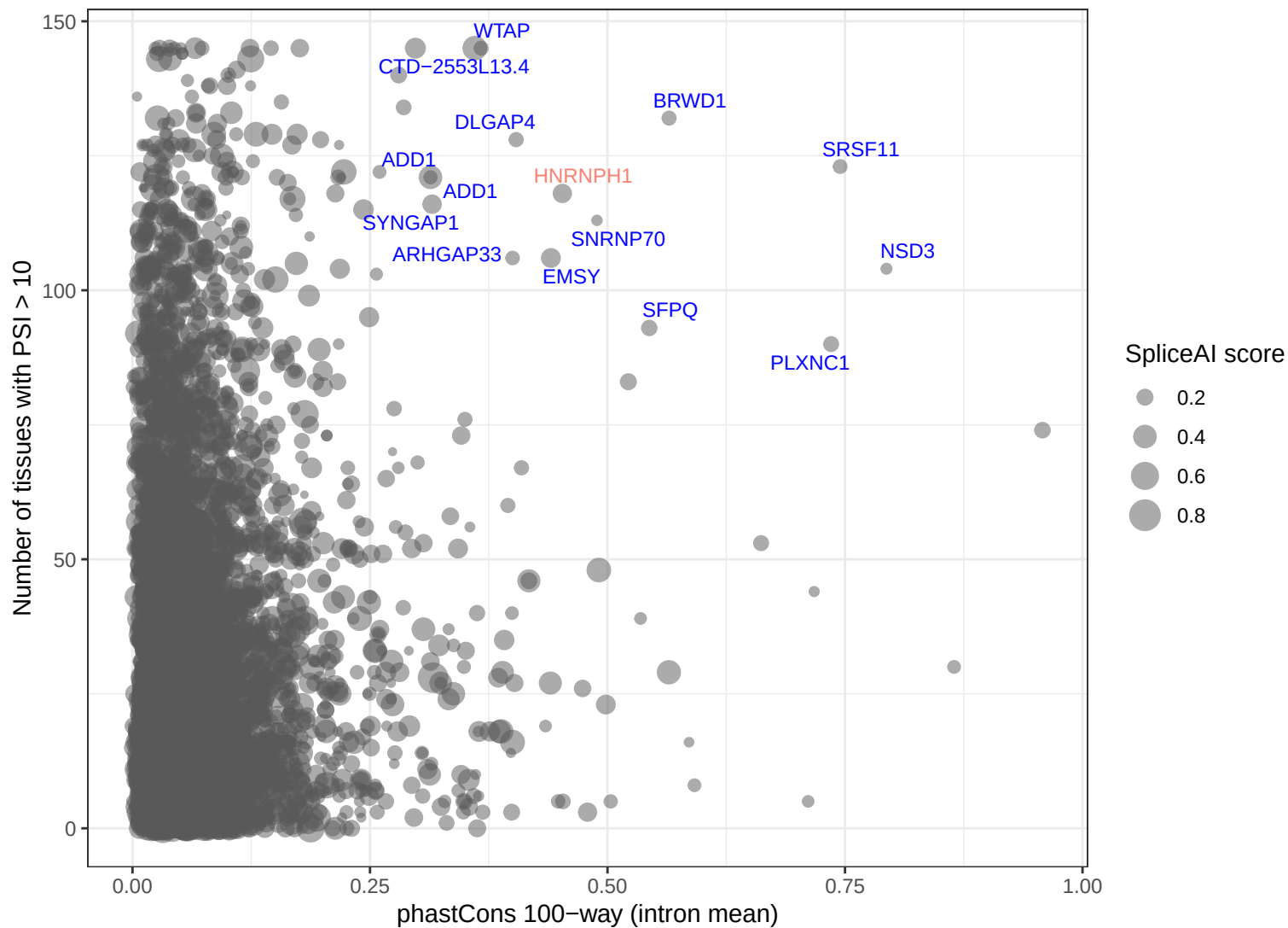
phastCons 100-way vs all Vast-DB tissues with PSI > 10
