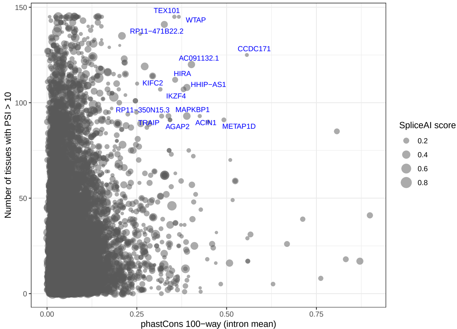
Supported cryptics: phastCons 100-way vs all Vast-DB tissues with PSI > 10
